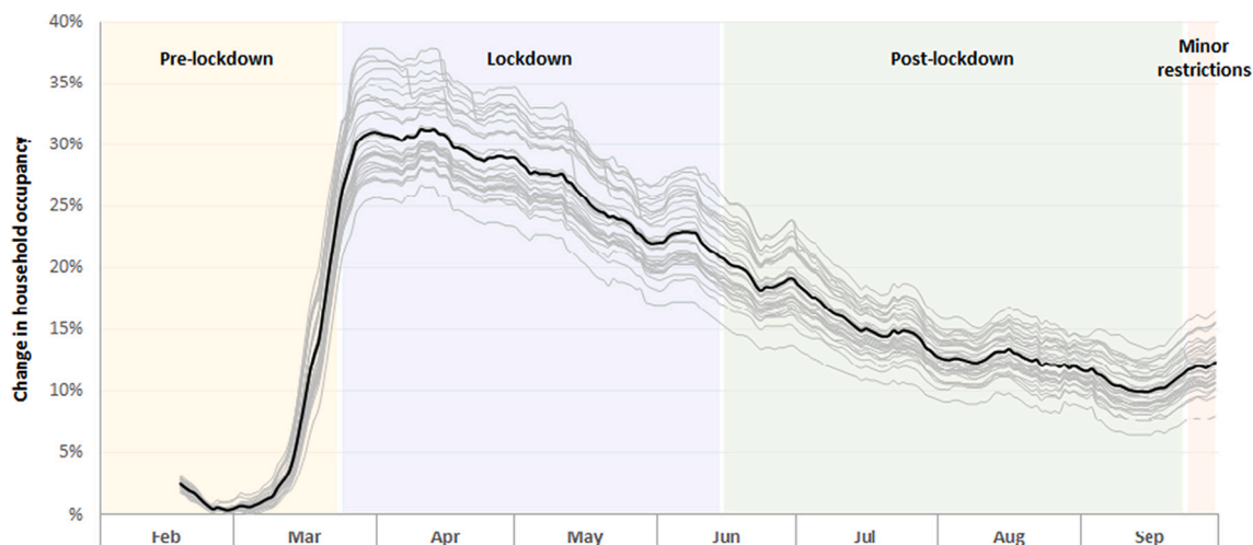
Fig. 1. Seven-day rolling average change in household occupancy (time spent at home) in 2020 (relative to the median level between January 3rd and February 6th that year) for each of the 33 London boroughs (grey) and the London average (black).
