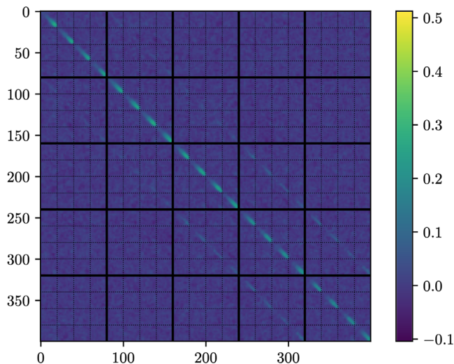
FIG. 13. Correlation matrix of the cross-component for the redMAGIC sample accounting for all lens-source pairs cross-covariance using 1799 lognormal simulations combined with jackknife resampling (see the text for details). The figure shows the correlation matrix minus its diagonal for illustrative purposes. Each one of the large squares corresponds to one of the five lens bins, while the small squares correspond to one of the four source bins. Beyond the autocorrelations in each lens-source pair, we can see that bin pairs sharing the same sources and with adjacent lens bins are also correlated.
