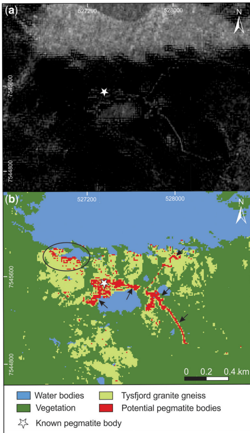
Fig. 5. Comparison between the conventional band ratio 4/12 method (a) and the support vector machine learning (SVM) algorithm (b) applied to Sentinel 2 images established for the Håkonhals area on the Finnøy island in Tysfjord, northern Norway. In (b) a new potential pegmatite (black circle) has been identified, as well as pegmatite mine dumps and roads paved with pegmatite gravel (black arrows). The applied projection is UTM/33N WGS84.
