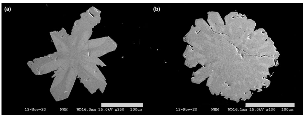
Fig. 4. Back-scattered electron images of two illoqite-(Ce) aggregates in ussingite showing the chemical heterogeneity (both images from sample KNR 44274). In both images the scale bar is 100 µm.
