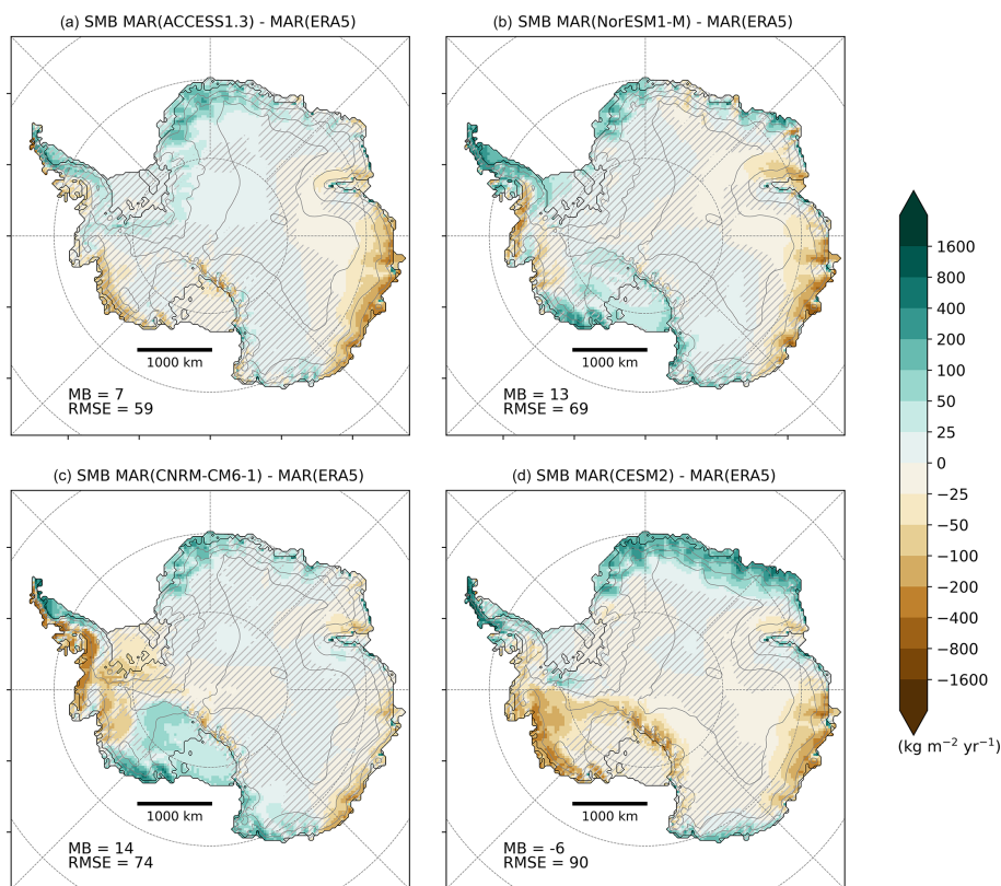
Figure 2. Comparison between the annual mean SMB simulated by MAR forced by ACCESS1.3 (a), NorESM1-M (b), CNRM-CM6-1 (c), and CESM2 (d) and the annual mean SMB simulated by MAR(ERA5) ( \text{kg m}^{-2} \text{yr}^{-1} ) over 1981–2010. Locations where anomalies are smaller than the (natural) interannual variability in the present climate (interannual standard deviation) are hatched. Mean bias (MB) and root mean square error (RMSE) compared to MAR(ERA5) are also indicated (units: \text{kg m}^{-2} \text{yr}^{-1} ).
