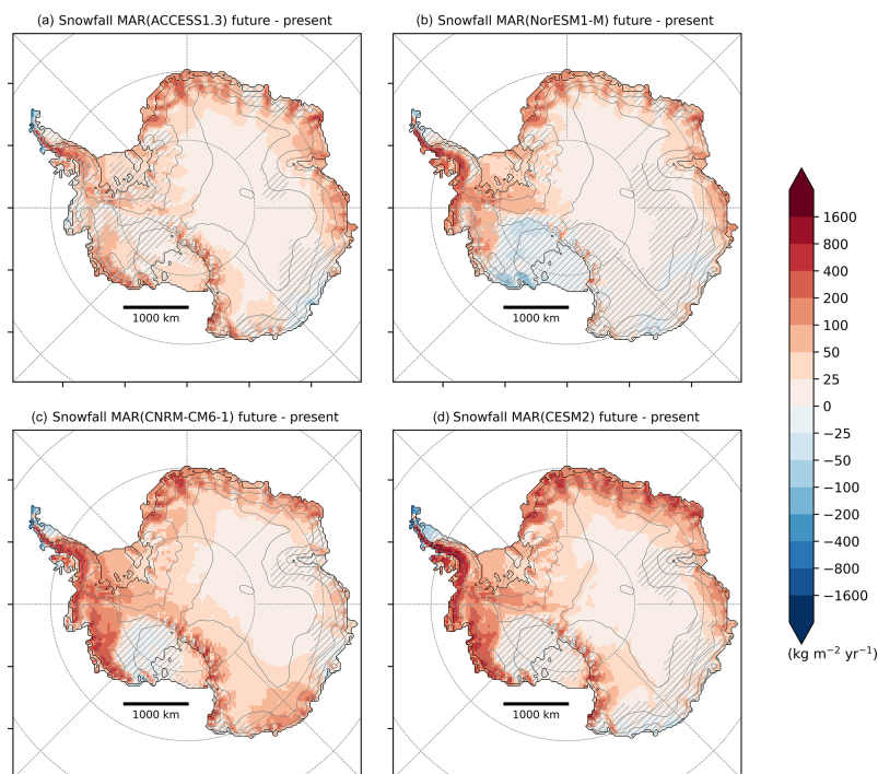
Figure 4. Snowfall changes ( \text{kg m}^{-2} \text{yr}^{-1} ) between 2071–2100 and 1981–2010 as modelled by MAR forced by ACCESS1-3 (a), NorESM1-M (b), CNRM-CM6-1 (c), and CESM2 (d) using ssp585 and RCP8.5. Locations where changes are smaller than the (natural) interannual variability in the present climate (interannual standard deviation) are hatched.
