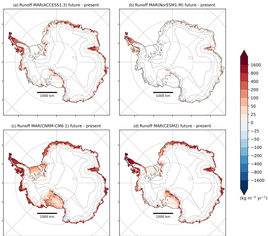
Figure 6. Changes in run-off production ( \text{kg m}^{-2} \text{yr}^{-1} ) between 2071–2100 and 1981–2010 as modelled by MAR forced by ACCESS1-3 (a), NorESM1-M (b), CNRM-CM6-1 (c), and CESM2 (d). Locations where changes are smaller than the (natural) interannual variability in the present climate (interannual standard deviation) are hatched.
