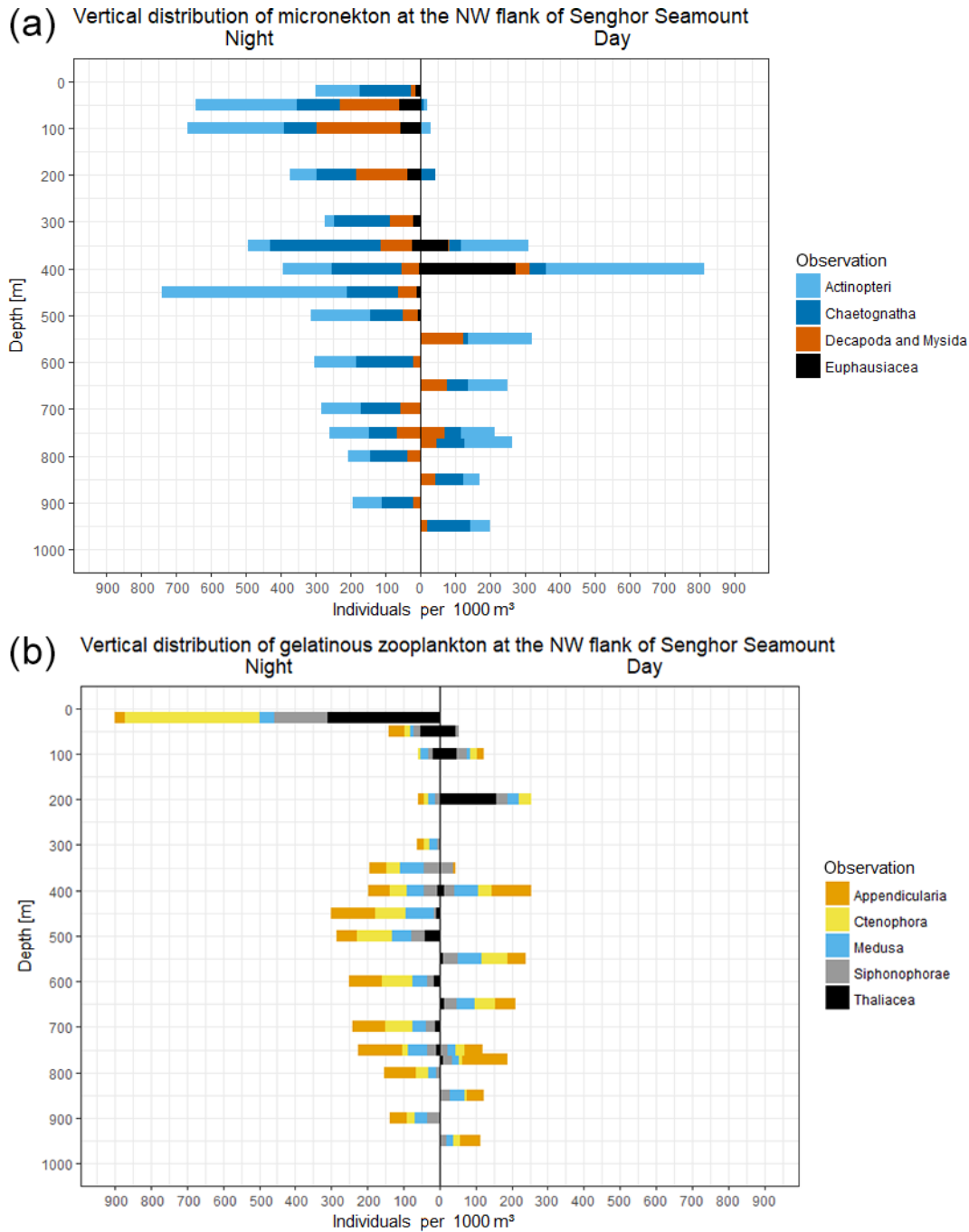
Figure 4. Day and night comparison of faunal observations obtained by PELAGIOS at the northwest flank of Senghor Seamount: (a) fishes, krill, chaetognaths, and decapods; (b) gelatinous zooplankton groups.
