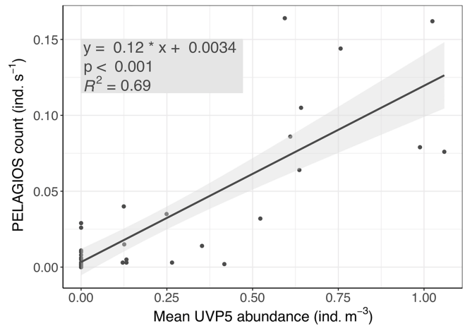
Figure 3. PELAGIOS video counts of Poeobius sp. as a function of UVP5-derived abundance on the same transects at two stations on cruise MSM 49 on R/V Maria S. Merian .
