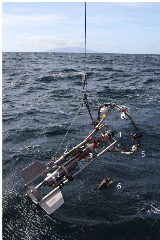
Figure 1. (a) The Pelagic In Situ Observations System (PELAGIOS) with battery (1), CTD (2), telemetry (3), camera (4), LEDs (5), and depressor (6) during deployment from R/V Poseidon in February 2018 (photo: Karen Hissmann).
