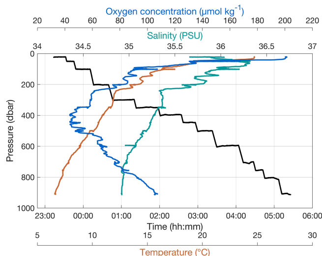
Figure 2. Stairwise trajectory of PELAGIOS through the water column, to the desired depths with concomitantly measured environmental data.
