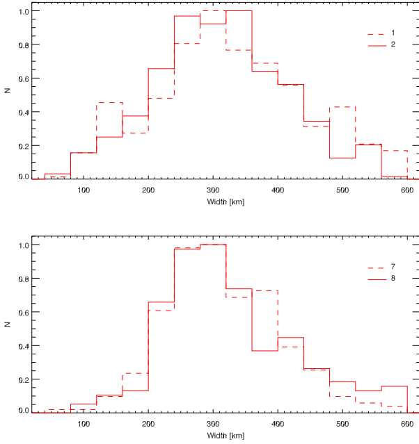
Fig. 14. Normalised histograms of the widths of the rain blobs determined for the density calculations from H \alpha . These widths are determined as explained in Sect. 4.2.1 and shown in Fig. 9. We only show the measurements that have an error below 15% of the measured value. Top: paths 1 and 2. The total number of rain blobs detected are, respectively, 533 and 450. Bottom: paths 7 and 8. The total number of rain blobs detected are, respectively, 283 and 213.
