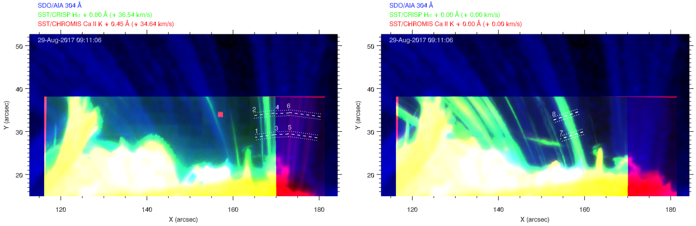
Fig. 7. Zoom on the coronal rain in the SST FOV. Images are stacked from 09:07:06 to 09:11:06 in order to highlight the display of the different bundles. The dashed lines show the different paths chosen for the analysis and the parallel dotted lines show the thickness covered by the slices constructed around these paths. Left: RGB image combining the AIA 304 Å in blue, red wing H \alpha in green, and red wing Ca II K in red. Right: same FOV with H \alpha line center in green and Ca II K line center in red.
