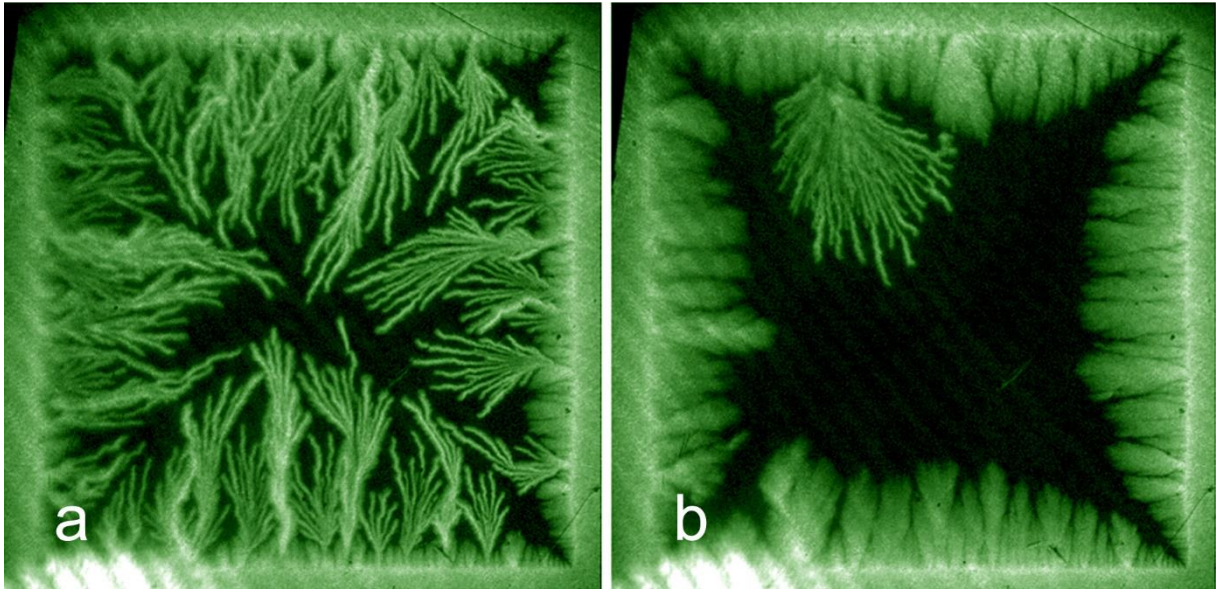
Figure 4. Flux penetration in the MgB 2 film exposed to magnetic field of 20 mT applied by using ramp rates of (a) 2700 T/s, and (b) 48 T/s. In both cases the sample was initially cooled to 12.5 K in zero magnetic field.
