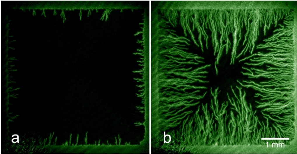
Figure 2. Magneto-optical images of the MgB 2 film after zero-field-cooling to 7 K and applying a gradually increasing field at a rate of 2 mT/s. The images in (a) and (b) show the flux penetration when the applied field reached 5 mT and 20 mT, respectively.
