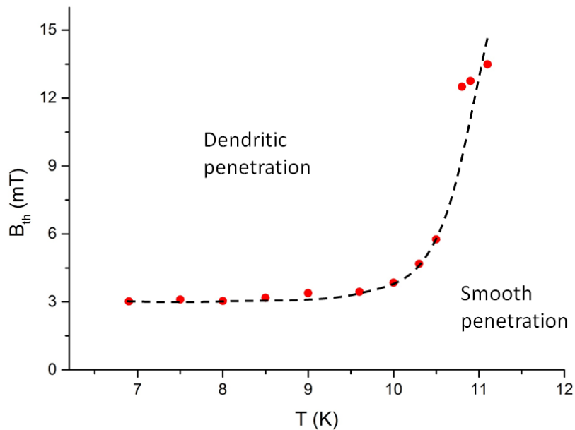
Figure 3. The threshold field, B_{th} , of the MgB 2 film as a function of sample temperature when a perpendicular field was ramped up at the rate of 2 mT/s. The dotted line is a guide to the eye. The film is stable at the conditions below this line.
