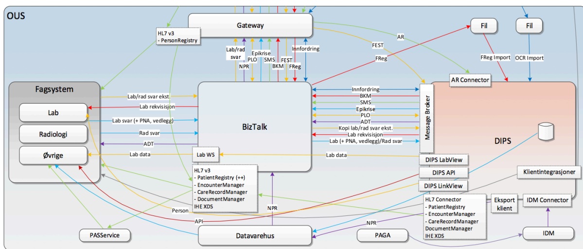
Figure 3: The Integration Platform at Oslo University Hospital (source: Digital Renewal Programme)
