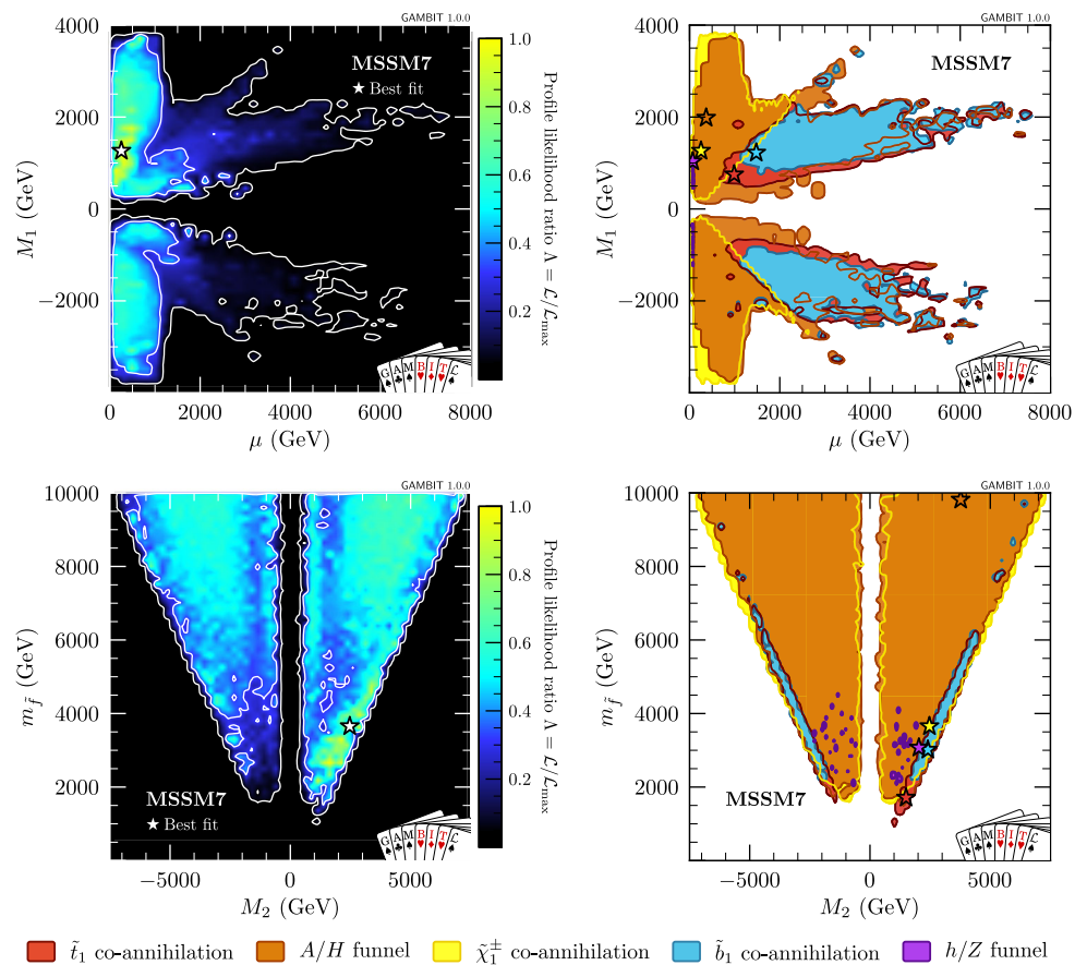
Fig. 3 Left: joint profile likelihoods in the \mu - M_1 (top) and M_2 - m_{\tilde{f}} planes (bottom). Stars indicate the point of highest likelihood in each plain, and white contours correspond to the 1\sigma and 2\sigma CL regions with respect to the best-fit point. Right: coloured regions indicating in which parts of the 2\sigma best-fit region different co-annihilation and funnel mechanisms contribute to keeping the relic density low. The best-fit point in each region is indicated by a star with the corresponding colour
