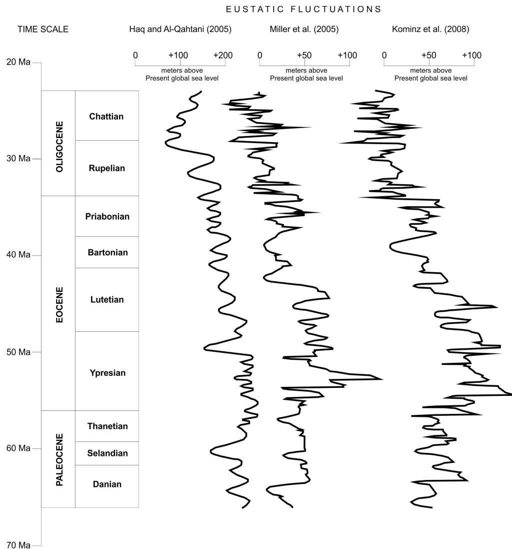
Fig. 1. The principal modern global sea-level curves. The geologic time scale follows Gradstein et al. (2012a); see also stratigraphy.org for updates. The original eustatic curves are re-scaled. Because of differences in the geologic time scales employed by different authors (see text for additional explanations), the depicted curves should not necessarily match at resolution higher than 5 (usually 1–2) Ma.
