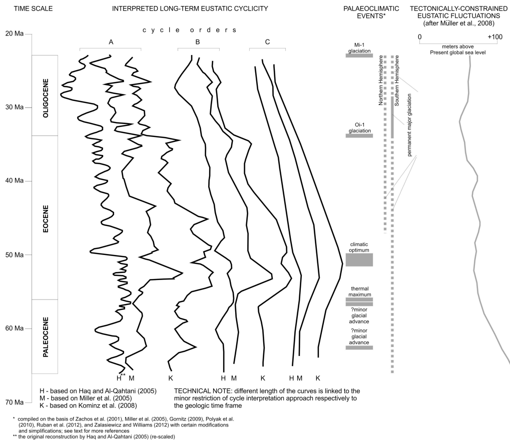
Fig. 2. Long-term eustatic cycle interpretations and the palaeoclimatic and tectonic evidence.
