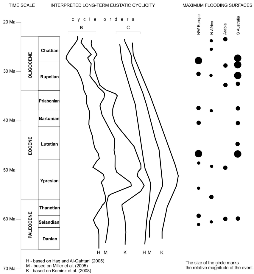
Fig. 3. Long-term eustatic cycle interpretations and regional major flooding surfaces (established provisionally on the basis of data from McGowran et al., 2004; Guiraud et al., 2005; Simmons et al., 2007; Gradstein et al., 2012). The simplified geologic time scale follows Gradstein et al. (2012).
