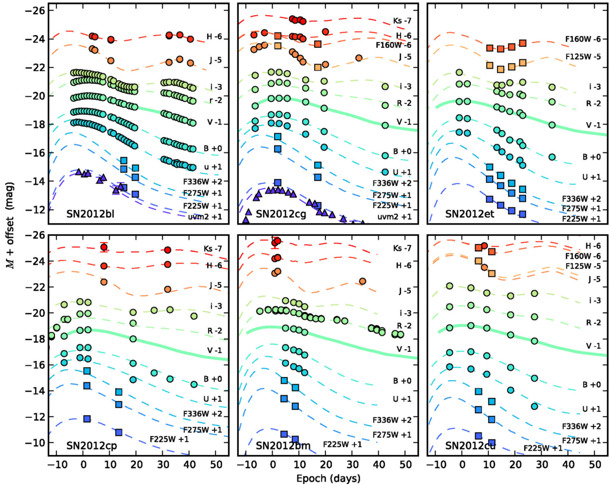
Figure 3. Observed light curves for the SN sample. Our analysis is based on optical UBVRI and NIR JHK photometry from ground-based observatories (circles), UV ( F225W , F275W , F336W ) and NIR ( F125W , F160W ) photometry from the HST (squares). For the SNe 2012bl and 2012cg we also use Swift /UVOT photometry (triangles). The data are shown in their instrumental system but have been shifted using the distance moduli based on the distances in Table 1 and offset for clarity. The thick, solid, lines show the SNOOPY V -models used to calculate colours as described in the text, while the dashed lines show synthesized light curves of SN 2011fe to guide the eye. When an SN has observations in a similar filter from multiple instruments only one of the light curves is shown. The epoch is the observed date with respect to the fitted day of maximum in the B band from Table 5.
