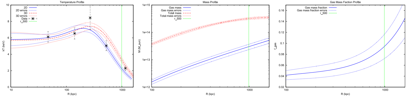
Figure 9. Temperature, gas mass and total mass, and gas mass fraction profiles for G036N obtained by XMM-Newton , with N_H = 0.136 \times 10^{22} \text{ cm}^{-2} (total value). The vertical green dashed line marks r_{500} for all three panels. Left: temperature profiles. The blue solid and blue dotted lines are the best-fitting 2D temperature profile and the corresponding 1\sigma errors, while the red dash-dotted and red short-dashed lines are the best-fitting 3D temperature profiles and the corresponding errors. The data points with errors are the measured 2D temperatures in each bin. Middle: gas mass and total mass profiles. The upper red dash-dotted and red short-dashed lines are the total mass profile and the corresponding errors, while the lower blue solid and blue dotted lines are the gas mass and the corresponding errors. Right: gas mass fraction profile. The blue solid and blue dotted lines are the gas mass fraction profile and the corresponding errors.
