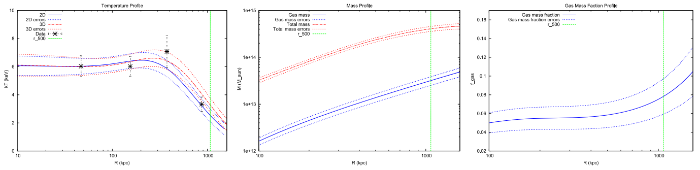
Figure 17. Same as Figure 9, except for Chandra baseline background model and N_H = 0.164 \times 10^{22} \text{ cm}^{-2} (best-fitting value).
