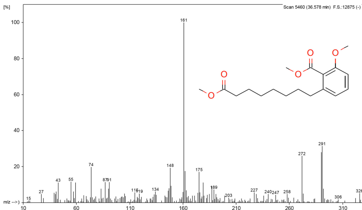
Figure 13 Mass spectrum and molecular structure for ebteric acid (methyl 2-methoxy-6-(8-oxooctyl)benzoate), an abundant marker in fully-cured CNSL.
