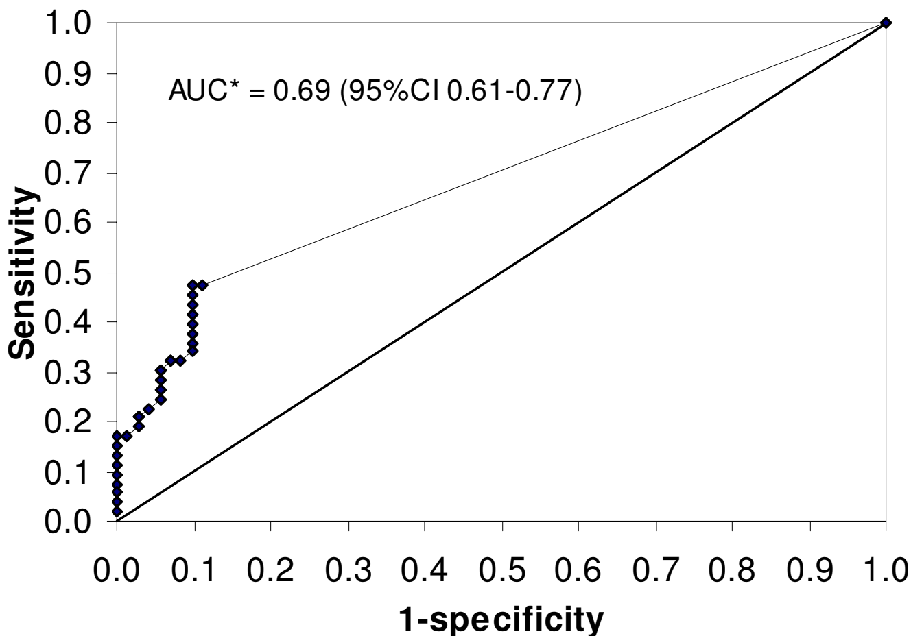
Figure 1 CMV quantitative PCR results expressed as ROC curve. Receiver operating characteristic (ROC) curve based on quantitative CMV PCR results in the last available plasma sample prior to the first diagnosis of CMV disease (alive or at autopsy) or death without CMV disease. *AUC = area under the curve.
