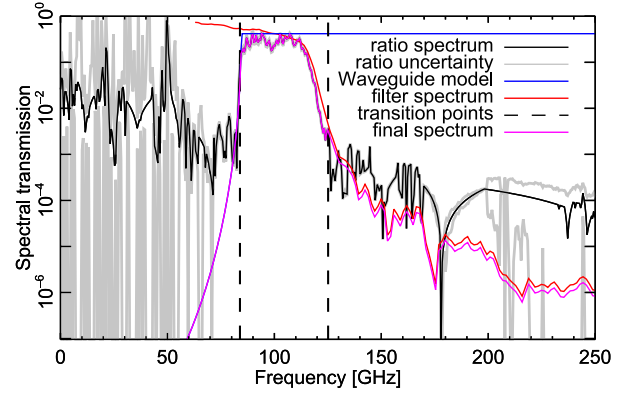
Fig. 4. Example ratioed spectrum (black), filter spectrum (red), waveguide model (blue), and final output spectral response (violet) for HFI 100 GHz detector 1a. The transition frequencies are shown by the vertical dashed lines. While the in-band spectral response is determined by the ratioed spectrum, the out-of-band transmission is determined by the waveguide model and filter data.
