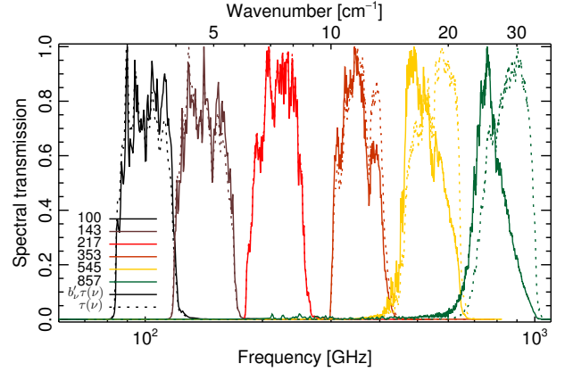
Fig. 14. Product of the HFI band-average spectra, \tau(\nu) , with the CMB dipole spectral profile, i.e., b'_\nu\tau(\nu) (Eq. (8)) shown using solid curves. The nominal spectra are shown as dotted curves for reference.
