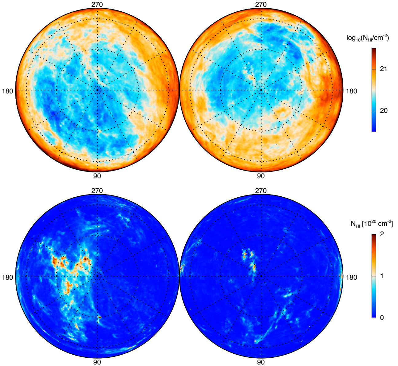
Fig. 2. Polar orthographic projections of the LVC map (upper) and the IVC map (lower) shown in Fig. 1. The left (right) panel is centred on the north (south) Galactic pole. Longitude increases clockwise (anticlockwise), with the two panels joining at l = 0^\circ and b = 0^\circ . Dotted lines representing constant longitude and latitude are spaced by 30^\circ . The radius from the pole is \propto \cos(b) , so this projection emphasizes features at high latitude.
