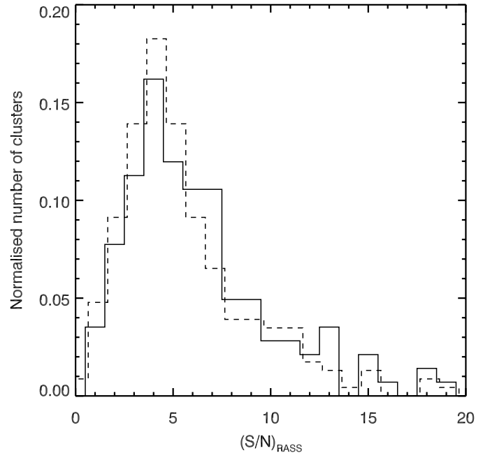
Fig. 17. Normalized distribution of the S/N in RASS at the position of Planck SZ detections with SDSS richness-based quality Q_{SDSS} = 1 (solid line) and Q_{SDSS} = 2 (dashed line).
