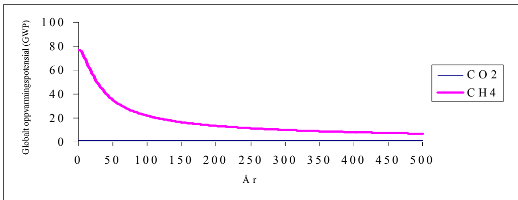
Figur 3. GWP for metan (CH 4 ) for ulike tidshorisonter. Kilde: Sygna et al. (1999).
