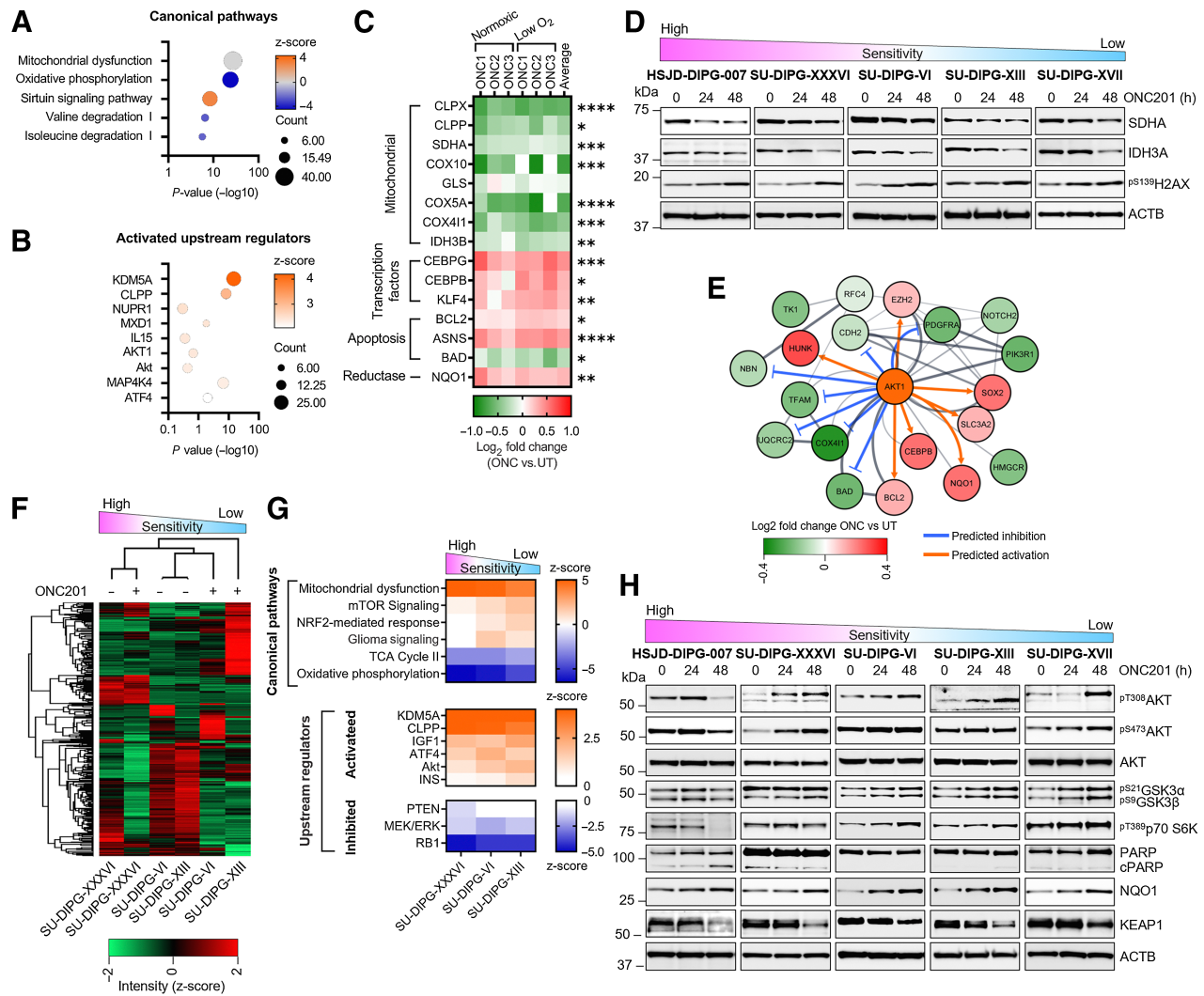
Figure 3. Quantitative proteomic profiling identifies increased PI3K/Akt signaling in resistant models. High-resolution quantitative proteomic profiling was conducted on SU-DIPG-VI, exposed to 5 \mu\text{mol/L} ONC201 for 24 hours. Cells were treated in low oxygen (5% \text{O}_2 , 5% \text{CO}_2 ) and normoxic conditions (20% \text{O}_2 , 5% \text{CO}_2 ) in biological triplicate. A and B , Major canonical pathways ( A ) and activated upstream regulators (determined by IPA; B ) of proteins significantly altered following 5 \mu\text{mol/L} ONC201, regardless of oxygen tension (Student t test, P < 0.05 , n = 6 ). C , Expression changes of proteins were calculated as \log_2 -fold change and grouped by mitochondrial proteins, transcription factors, and protein markers of apoptosis. Student t test of average change; *, P < 0.05 ; **, P < 0.01 ; ***, P < 0.001 ; ****, P < 0.0001 . D , Orthogonal validation of mitochondrial changes, such as decreased SDHA, was analyzed in DIPG cell lines (HSJD-DIPG-007, SU-DIPG-XXXVI, SU-DIPG-VI, SU-DIPG-XIII, and SU-DIPG-XVII) via Western blot, exposed to 5 \mu\text{mol/L} ONC201 for up to 48 hours. E , Network of proteins from upregulated PI3K/Akt signaling predicted by IPA were integrated in Cytoscape StringApp. Predicted increase (orange) and predicted decrease (blue) functional networks indicated with sharp and dark lines linking proteins to indicate a higher confidence interval. Protein expression changes mapped as \log_2 -fold change of ONC201/untreated calculated using the right-tailed Fisher exact test with the smaller the P value, the more likely the association between proteins not to be a random event ( P < 0.05 ). F and G , High-resolution quantitative proteomic profiling was conducted on SU-DIPG-XXXVI, SU-DIPG-VI and SU-DIPG-XXXVI, exposed to 5 \mu\text{mol/L} ONC201 for 24 hours. F , Heatmap and unbiased hierarchical clustering of protein expression values normalized using z-score of abundances in Perseus. G , Canonical pathways and predicted upstream regulators determined by IPA analysis of proteins altered following ONC201 exposure. Positive z-score value is predictive of pathway activation, whereas a negative z-score is predictive of inhibition. H , Orthogonal validation of protein-associated PI3K/Akt/mTOR signaling and the antioxidant-response element (ARE) axis were assessed in DIPG cell lines following ONC201 exposure.
