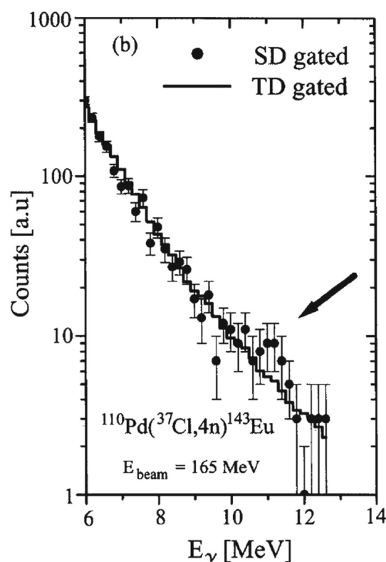
Fig. 8 GDR gated on SD discrete transitions; the figure was taken from reference [108] The figure is reproduced with permission from [108], © 2001, by Elsevier
