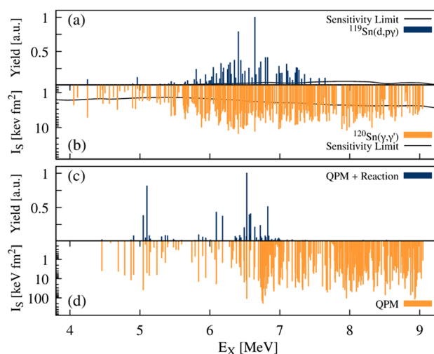
Fig. 4 a Relative \gamma -ray yields from ^{119}\text{Sn}(\text{d},\text{p}\gamma) and b energy-integrated cross sections I_S for ^{120}\text{Sn}(\gamma, \gamma') reactions. The corresponding theoretical results are displayed in (c) and (d) . Reprinted with permission from Ref. [41]. Copyright (2022) by the American Physical Society
