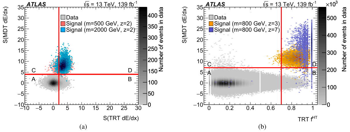
Fig. 4. (a) S(\text{MDT } dE/dx) versus S(\text{TRT } dE/dx) (used for the z=2 search) and (b) S(\text{MDT } dE/dx) versus \text{TRT } f^{\text{HT}} (used for the z > 2 search). The distributions of the data and the simulated signal samples (for charges z=2, 3 , and 7 , and masses of 500, 800 , and 2000 GeV) are shown. The signal distributions for the lowest MCP mass (a) or charge (b) are partially covered by the other signal distributions. D is the signal region and other regions are used to estimate the background contribution in that region (see text). Regions 0.01 < \text{TRT } f^{\text{HT}} < 0.02 , 0.49 < \text{TRT } f^{\text{HT}} < 0.50 , and 0.98 < \text{TRT } f^{\text{HT}} < 0.99 in (b) are underpopulated because \text{TRT } f^{\text{HT}} is a ratio of two integers belonging to the range of 0–50.
