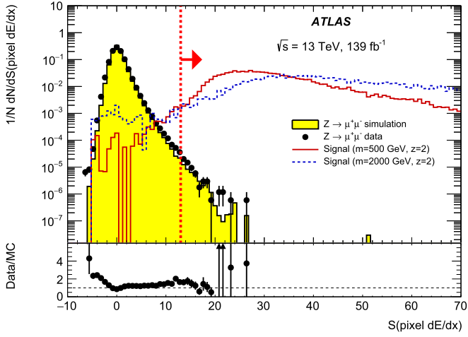
Fig. 2. Normalized distributions of the dE/dx significance in the pixel system, S(\text{pixel } dE/dx) , for muons from Z \rightarrow \mu\mu events (data and simulation) and for simulated MCPs passing the preselection requirements. Signal distributions are shown for z = 2 and masses of 500 and 2000 GeV. The vertical dotted line indicates the threshold of the tight selection criterion. A bin-by-bin ratio of Z \rightarrow \mu\mu distributions in data and simulation is shown on the lower panel. The arrows in the ratio plot are for points that are outside the range.
