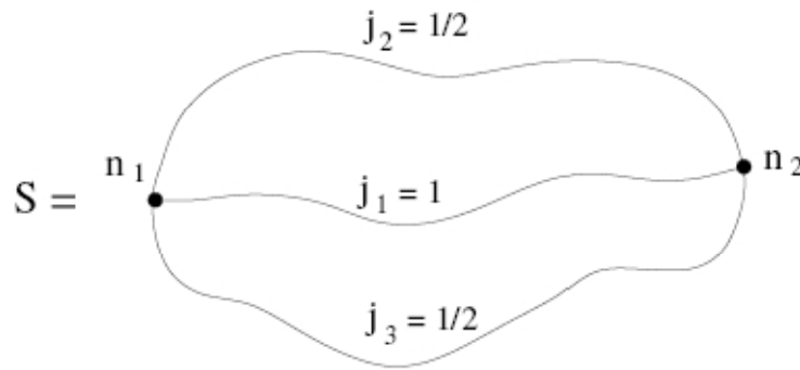
Figure 3.1. A spin network [From Rovelli (2004), p. 235].
