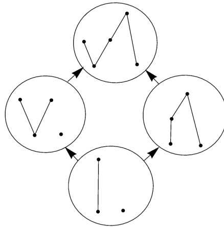
Figure 4.4. The principle of discrete general covariance.
