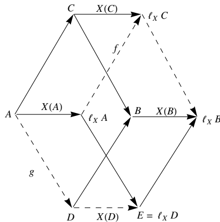
Figure 4.2. Weak translatability of an arrow field.
