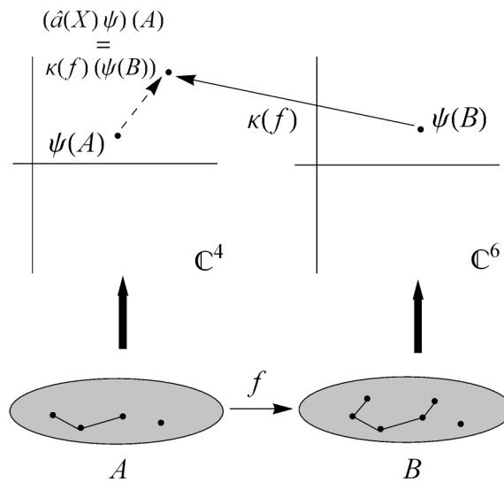
Figure 4.7. Representation of arrows by \kappa .
