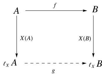
Figure 4.3. Completeness of an arrow field.
