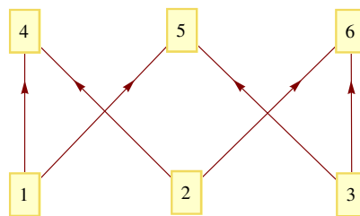
Figure 1.2. The "crown" causet.
