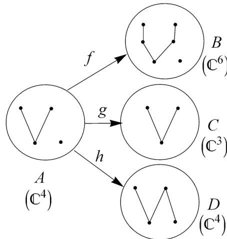
Figure 4.6. Object and arrow domain of the multiplier \kappa .
