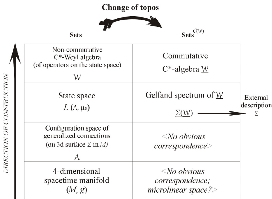
Figure 3.2. The Bohrification of LQG.
