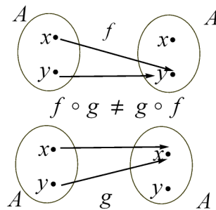
Figure 4.1. Noncommutativity of arrows.
