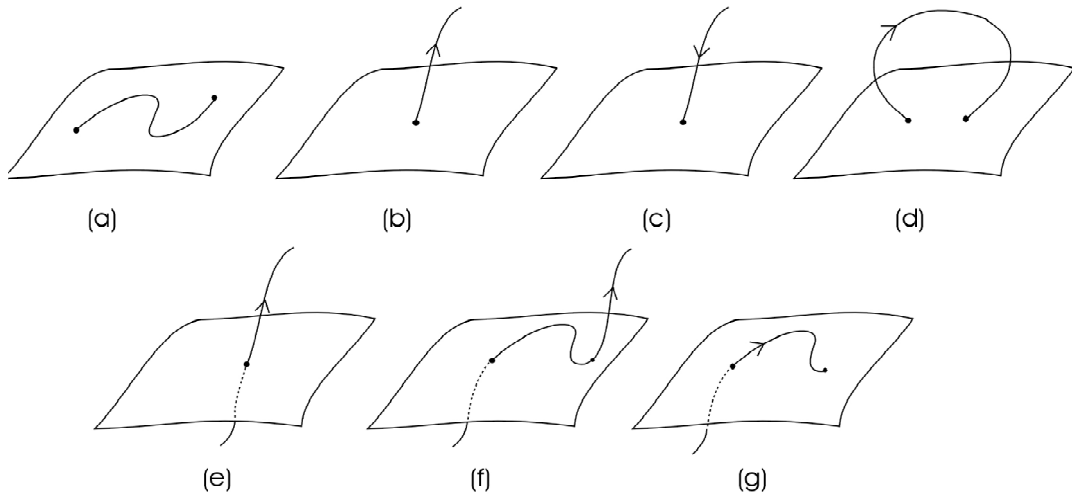
Figure 3.3. Some combinations of surfaces and paths.
