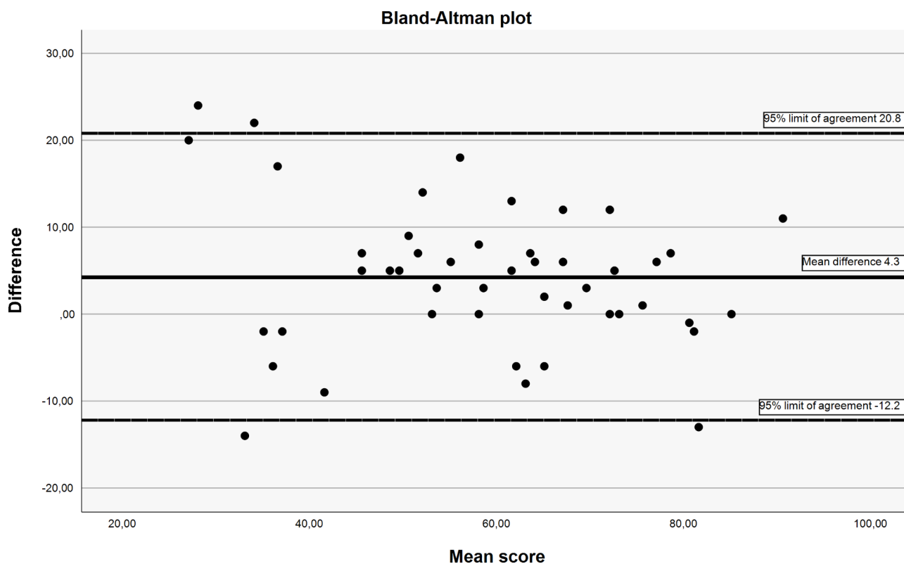
Fig. 2 Bland-Altman plot. Illustrating the VISA-G-Norwegian mean difference of 4.3 and the 95% limits of agreement at -12.2, 20.8
