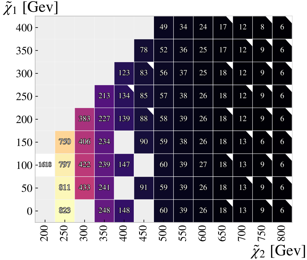
Figure 3.1: A grid of all chargino and neutralino mass combinations and their respective event count in the full signal data set. Additionally, a white corner has been added to all combinations which define the original signal set.
