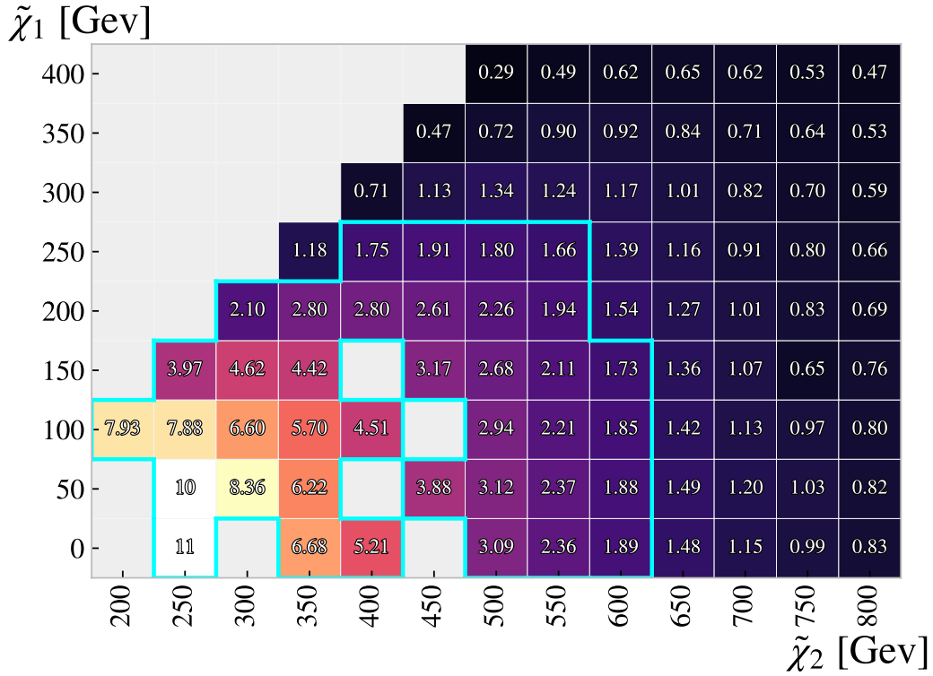
Figure 4.22: A grid displaying the expected significance on the complete signal grid using the signal region created by the maxout network. A band around each cell with a significance over 1.64 has been included.
