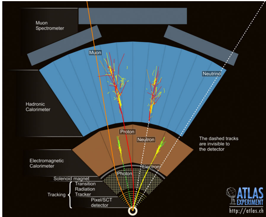
Figure 1.1: Event Cross-Section in a computer generated image of the ATLAS detector [22].
