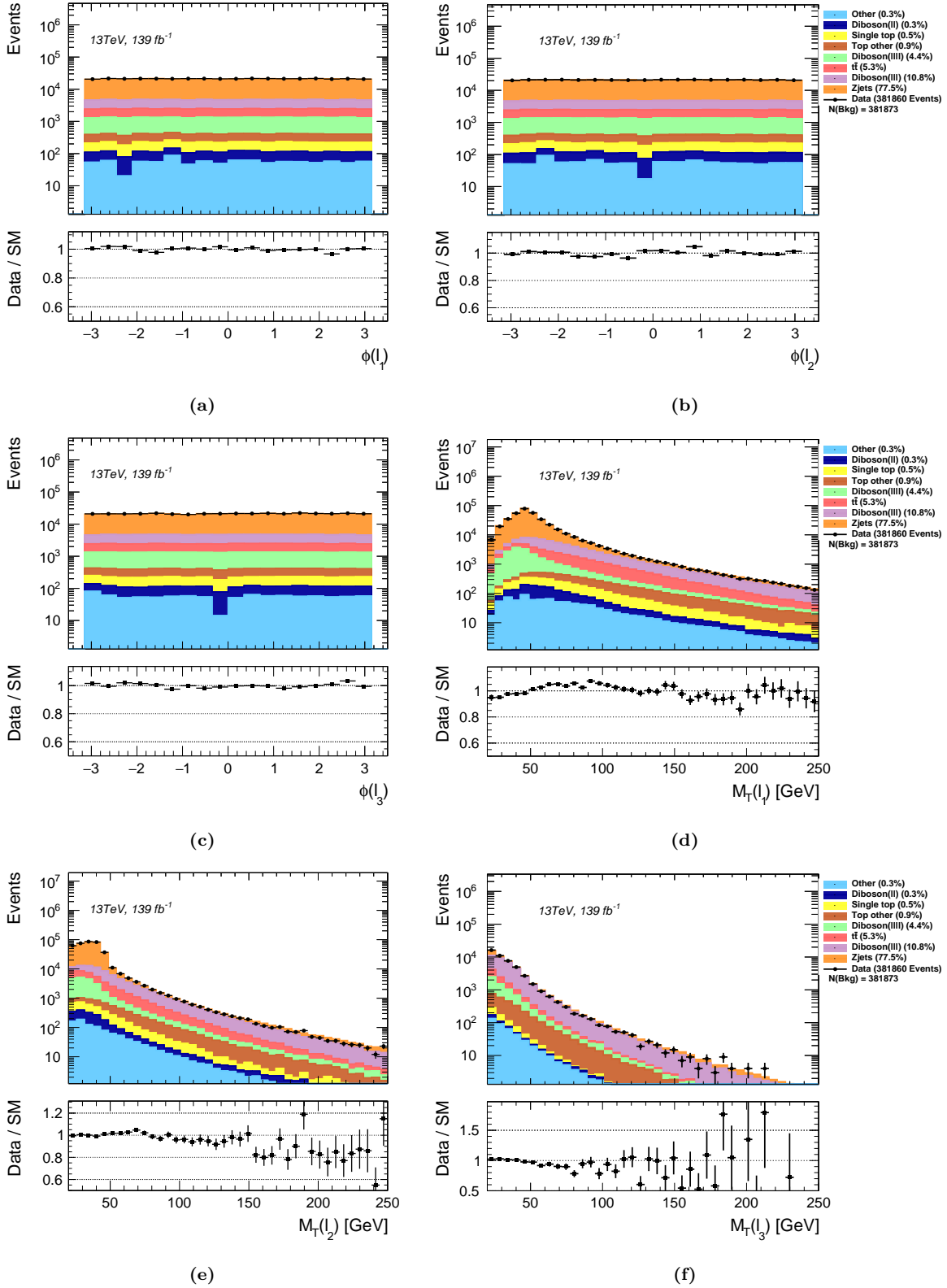
Figure 35: MC simulated and measured data comparison showing the \phi for the first 35a, second 35b and third 35c lepton. Similarly, the distribution over M_T for the first 35d, second 35e and third 35f lepton.
