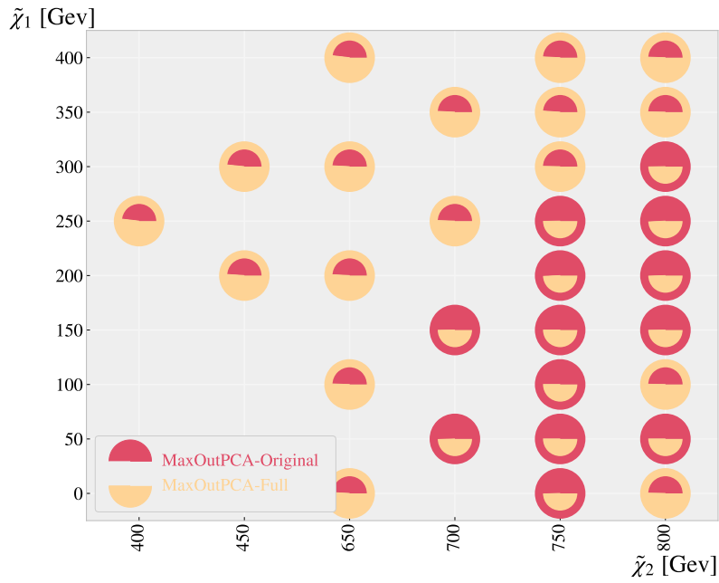
Figure 31: 'Pie-plot' comparing sensitivity achieved by the maxout model on the original signal set, where the figure shows the comparison between a model trained on the original signal grid, and the complete signal grid. A PCA analysis has been applied to the data being utilized in this result. The size of each 'slice' represents the relative size of the significance and the color around each point displays the method with the largest sensitivity for the respective combination.
