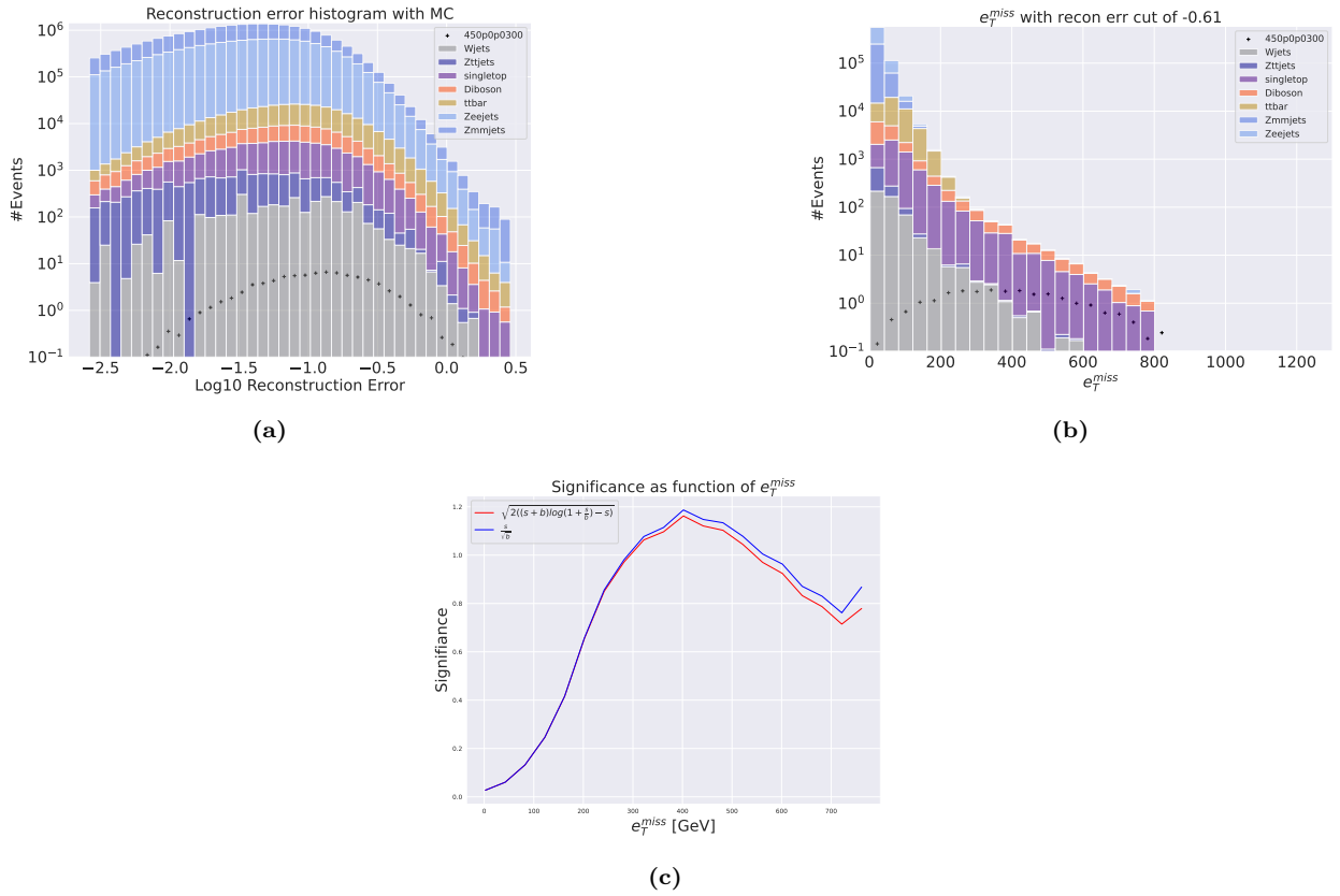
Figure 39: Reconstruction error (a), e_T^{\text{miss}} signal region (b) and significance as function of e_T^{\text{miss}} (c) for the deep regular autoencoder using SUSY 450p300. (a) shows that the peak of the distribution is somewhat centered in the middle of the reconstruction error range forming a bell-like shape. The peaks of the background and signal distributions are not well separated, with almost identical reconstruction error pattern. (b) shows a signal region with large background distribution. The signal region is made using a cut around 10^{-0.81} . The peaks in the signal region are also somewhat separated, but the overall distributions are overlapping still. (c) shows the significance as function of e_T^{\text{miss}} . The peak significance is around 1.2 at around 400 GeV.
