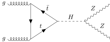
Figure 3.9: Proton-proton collision showing the Higgs channel. Here the Z bosons decay leptonically, leading to a four lepton final state.
