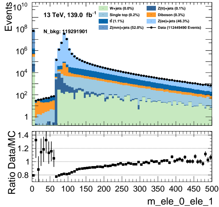
(b) Invariant mass for the first and second electron in GeV. The histogram contains the entire Run 2 dataset. Note the sharp reduction of events from 10-70 GeV.
