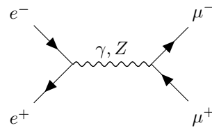
Figure 2.2: Feynman diagram of muon pair production from electron annihilation. Here, both Z and \gamma can work as the propagator.
