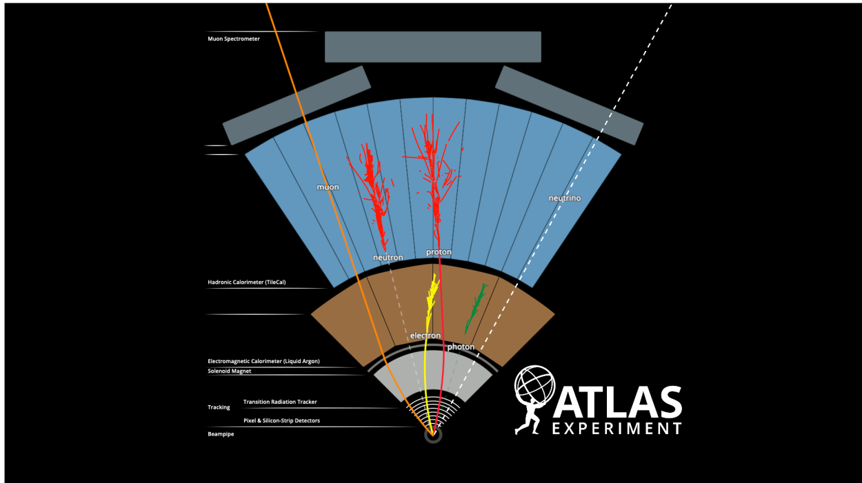
Figure 3.2: Figure describing how particles are detected at ATLAS, fetched from ATLAS detector slice (and particle visualisations) , by Sascha Mehlhase [25].
