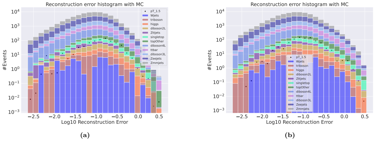
Figure 11: Reconstruction error on validation SM MC from the small (a) and large (b) variational autoencoder. The signal is a subsample of the validation set where the transverse momentum of the first electron and the first muon has been increased with a scale of 1.5. The change of transverse energy has also been changed according to the scaling of transverse momentum. A small peak is found around 10^{-0.8} .
