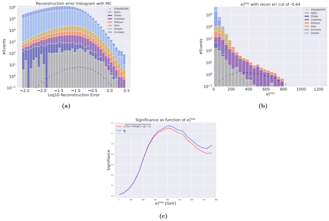
Figure 40: Reconstruction error (a), e_T^{miss} signal region (b) and significance as function of e_T^{miss} (c) for the deep regular autoencoder using SUSY 450p300. (a) shows that the peak of the distribution is somewhat centered in the middle of the reconstruction error range forming a bell-like shape. The peaks of the background and signal distributions are not well separated, with almost identical reconstruction error pattern. (b) shows a signal region with large background distribution. The signal region is made using a cut around 10^{-0.61} . The peaks in the signal region are also somewhat separated, but the overall distributions are overlapping still. (c) shows the significance as function of e_T^{miss} . The peak significance is around 1.31 at around 400 GeV.
