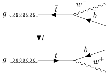
Figure 2.5: Proton-proton collision showing the t\bar{t} channel. Read from left to right.
