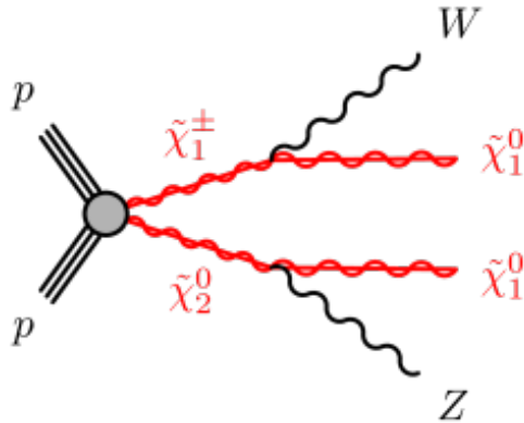
Figure 2.6: SUSY diagram showing chargino-neutralino production in proton-proton collision. The test samples we look for with this signal is where the W and Z boson decay leptonically.
