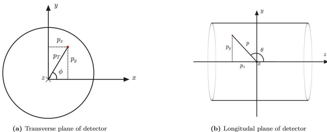
Figure 3.1: Spherical coordinate definitions with the azimuthal and polar angles \phi and \theta . Here figure 3.1a of the transverse plane shows the z-axis into the paper, where as figure 3.1b of the longitudinal plane shows the positive x-axis going out of the paper. Figure taken from [23].
