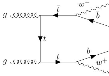
Figure 3.8: Proton-proton collision showing the t\bar{t} channel. Here the w bosons decay leptonically and one or more jets can be misreconstructed as fake leptons by the detector.
