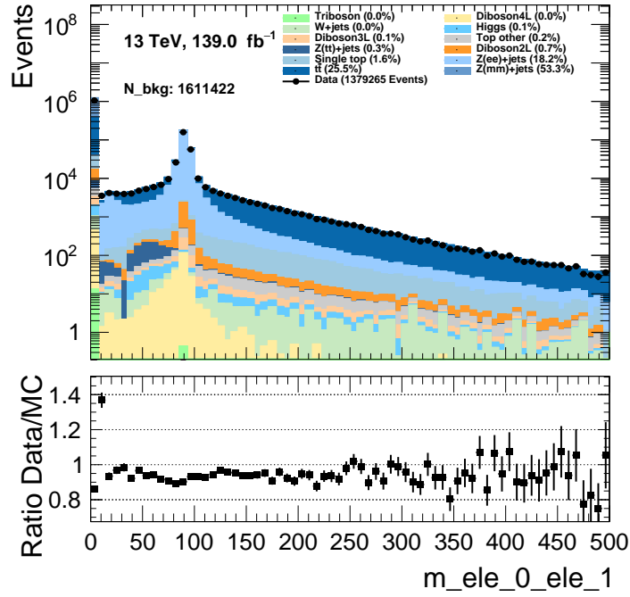
(b) Invariant mass for the first and second electron in GeV. The histogram contains the entire Run 2 dataset.
