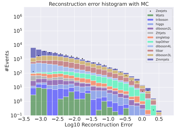
(b) Reconstruction error on validation SM MC from the big Autoencoder. Here the Zeejets channel has been removed from training and is used as signal. No significant difference in distributions is found.
