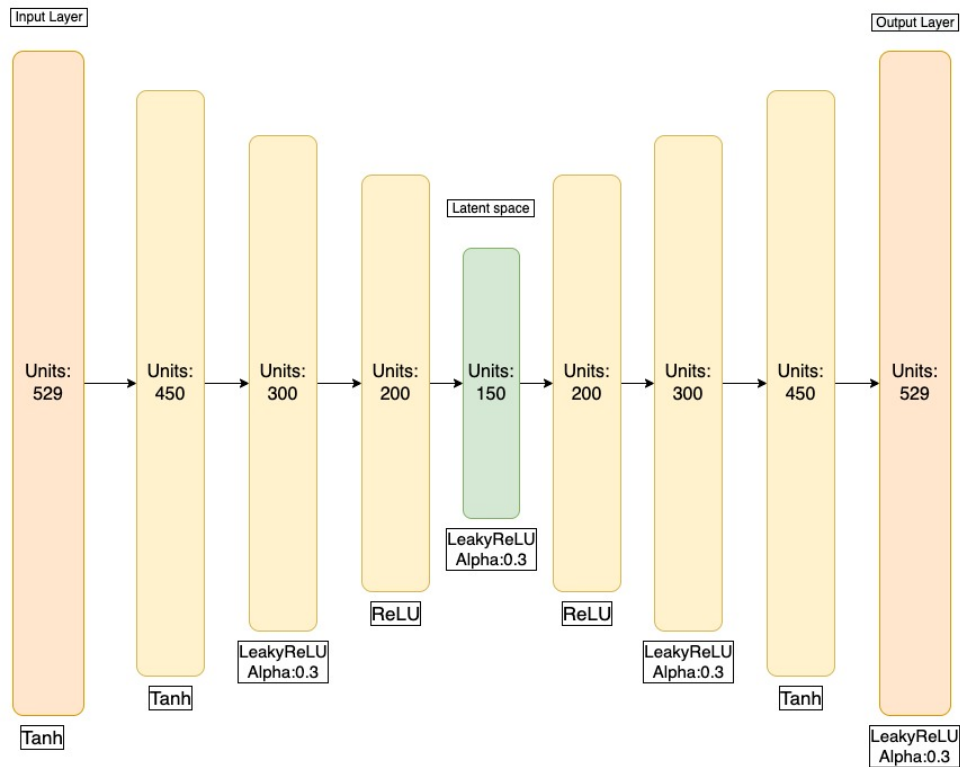
Figure 3.19: Large autoencoder architecture.
