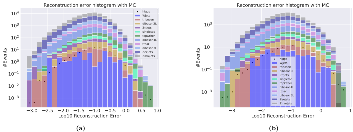
Figure 4.4: Reconstruction error on validation SM MC from the small (a) and large (b) variational autoencoder. The Higgs channel has been removed from training and is used as signal. No significant difference in distributions is found.
