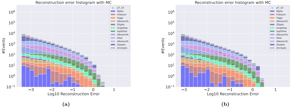
Figure 4.7: Reconstruction error on validation SM MC from the small (a) and large (b) regular autoencoder. The signal is a subsample of the validation set where the transverse momentum of the first electron and the first muon has been increased with a scale of 10. The difference in transverse energy between the objects has also been changed according to the scaling of transverse momentum. A peak is found around 10^{-1.6} .
