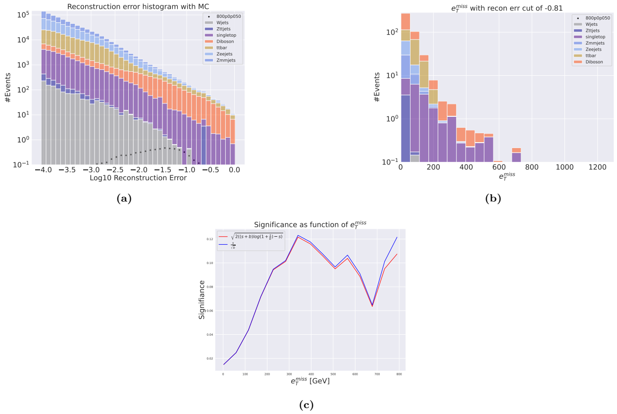
Figure 38: Reconstruction error (a), e_T^{miss} signal region (b) and significance as function of e_T^{miss} (c) for the deep regular autoencoder using SUSY 800p50. (a) shows the reconstruction error distribution for the SM MC and the SUSY signal. The autoencoder produces a slope like shape that is highly shifted to the lower end of the reconstruction error range for the background. The signal is more evenly spread out along the x-axis. The peaks of the two distributions are totally separated with two orders of magnitude in reconstruction error. (b) shows the e_T^{miss} T distribution for the SM MC and the SUSY signal in the signal region. The signal region is made using a cut around 10^{-0.81} . Most of the background is removed, and the peaks of the SM MC and signal distributions are somewhat separated. (c) shows the significance as function of e_T^{miss} . The peak is put around a cut of about 340 GeV in the e_T^{miss} , with a significance of around 0.125.
