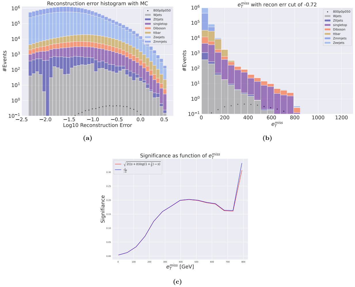
Figure 4.23: Reconstruction error (a), e_T^{miss} signal region (b) and significance as function of e_T^{miss} (c) for the deep variational autoencoder using SUSY 800p50. (a) shows that the peak of the distribution is somewhat centered in the middle of the reconstruction error range forming a hill-like shape. The peaks of the background and signal distributions are not well separated, with some separation of distribution peaks. (b) shows a signal region with large background distribution. The signal region is made using a cut around 10^{-0.72} . The peaks in the signal region are also somewhat separated, but the overall distributions are overlapping still. (c) shows the significance as function of e_T^{miss} . The peak significance is around 0.20 at around 450 GeV.
