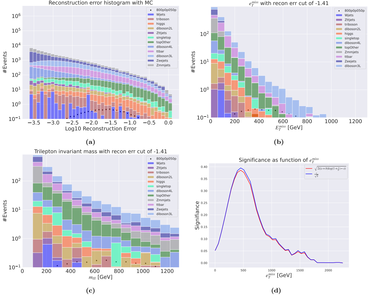
Figure 4.12: Reconstruction error, e_T^{miss} signal region, m_{III} signal region and significance as function of e_T^{miss} for the shallow regular autoencoder using the SUSY 800p50. Figure 4.12a shows the reconstruction error distribution for the SM MC and the SUSY signal. Here the autoencoder produces a mirrored reconstruction error shape for background and signal. The peaks of the two distributions are separated with two orders of magnitude in reconstruction error. Figure 4.12b shows the e_T^{miss} distribution for the SM MC and the SUSY signal in the signal region, defined as the region having a \log_{10} reconstruction error above -1.41. Most of the background is removed, and the peaks of the SM MC and signal distributions are separated. Figure 4.12c shows the m_{III} distribution for the SM MC and the SUSY signal. The shape of the SM MC and the signal distributions are somewhat separated. Figure 4.12d shows the significance as function of e_T^{miss} . The maximum significance is found when applying a cut of about > 450 GeV in the e_T^{miss} , with a significance of around 0.39.
