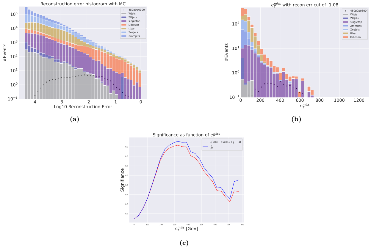
Figure 31: Reconstruction error (a), e_T^{miss} signal region (b) and significance as function of e_T^{miss} (c) for the deep regular autoencoder using SUSY 450p300. (a) shows the reconstruction error distribution for the SM MC and the SUSY signal. The autoencoder produces a slope like shape that is highly shifted to the lower end of the reconstruction error range for the background. The signal is more evenly spread out along the x-axis. The peaks of the two distributions are totally separated with two orders of magnitude in reconstruction error. (b) shows the e_T^{miss} T distribution for the SM MC and the SUSY signal in the signal region. The signal region is made using a cut around 10^{-1.08} . Most of the background is removed, and the peaks of the SM MC and signal distributions are somewhat separated. (c) shows the significance as function of e_T^{miss} . The peak is put around a cut of about 340 GeV in the e_T^{miss} , with a significance of around 0.95.
