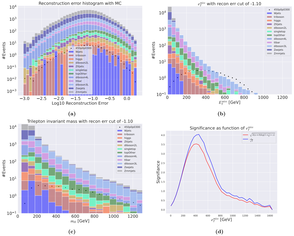
Figure 4.13: Reconstruction error, e_T^{miss} signal region, m_{III} signal region and significance as function of e_T^{miss} for the deep variational autoencoder using the SUSY 450p300. Figure 4.13a shows the reconstruction error distribution for the SM MC and the SUSY signal. Here the autoencoder produces a hill-like for background and signal with little distinction. The peaks of the two distributions are not separated in reconstruction error. Figure 4.13b shows the e_T^{miss} distribution for the SM MC and the SUSY signal in the signal region, defined as the region having a \log_{10} reconstruction error above -1.10. Some background is removed, and the peaks of the SM MC and signal distributions are separated. Figure 4.13c shows the m_{III} distribution for the SM MC and the SUSY signal. The shape of the SM MC and the signal distributions are displaying almost the same shape. Figure 4.13d shows the significance as function of e_T^{miss} . The maximum significance is found when applying a cut of about > 450 GeV in the e_T^{miss} , with a significance of around 4.1.
