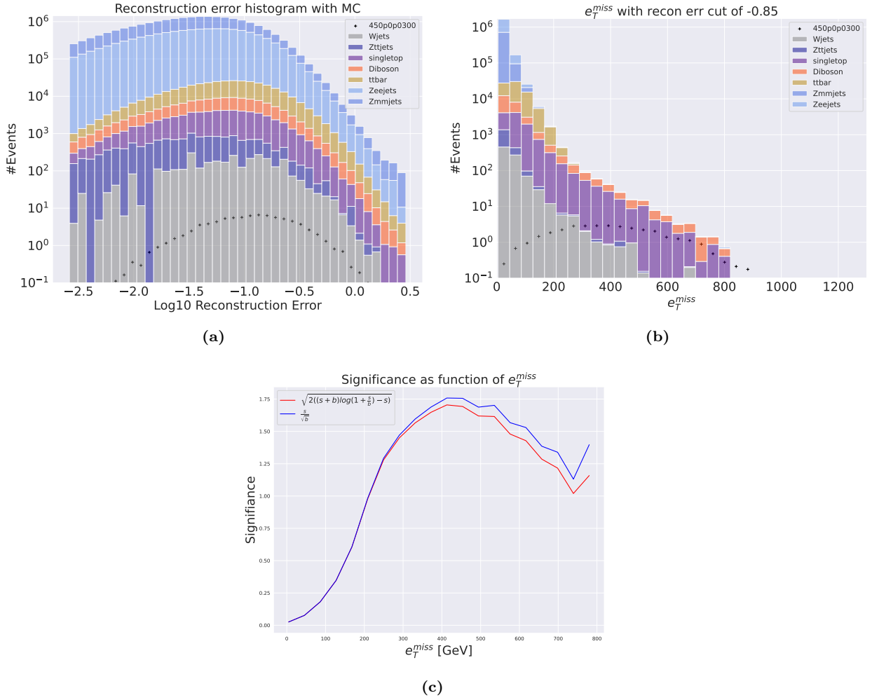
Figure 4.22: Reconstruction error (a), e_T^{miss} signal region (b) and significance as function of e_T^{miss} (c) for the shallow variational autoencoder using SUSY 450p300. (a) shows that the peak of the distribution is somewhat centered in the middle of the reconstruction error range forming a hill-like shape. The peaks of the background and signal distributions are not well separated, with almost identical reconstruction error pattern. (b) shows a signal region with large background distribution. The signal region is made using a cut around 10^{-0.85} . The peaks in the signal region are also somewhat separated, but the overall distributions are overlapping still. (c) shows the significance as function of e_T^{miss} . The peak significance is around 1.75 at around 420-450 GeV.
