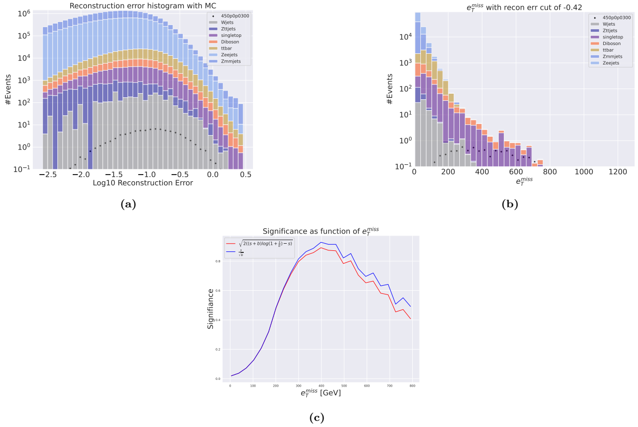
Figure 44: Reconstruction error (a), e_T^{miss} signal region (b) and significance as function of e_T^{miss} (c) for the deep regular autoencoder using SUSY 450p300. (a) shows that the peak of the distribution is somewhat centered in the middle of the reconstruction error range forming a bell-like shape. The peaks of the background and signal distributions are not well separated, with almost identical reconstruction error pattern. (b) shows a signal region with large background distribution. The signal region is made using a cut around 10^{-0.42} . The peaks in the signal region are also somewhat separated, but the overall distributions are overlapping still. (c) shows the significance as function of e_T^{miss} . The peak significance is around 0.92 at around 400 GeV.
