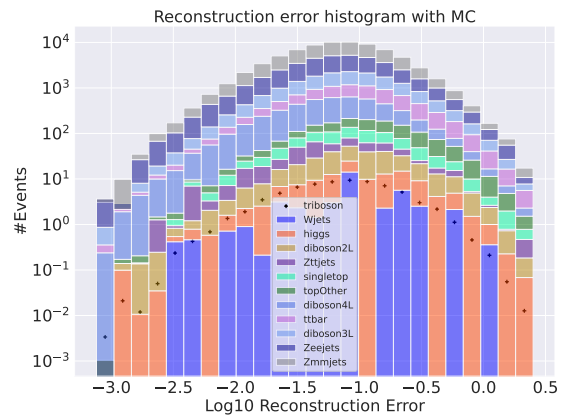
(f) Reconstruction error on validation SM MC from the big Autoencoder. Here the triboson channel has been removed from training and is used as signal. No significant difference in distributions is found.
