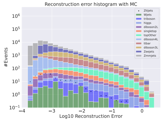
(f) Reconstruction error on validation SM MC from the big Autoencoder. Here the Zttjets channel has been removed from training and is used as signal. No significant difference in distributions is found.
