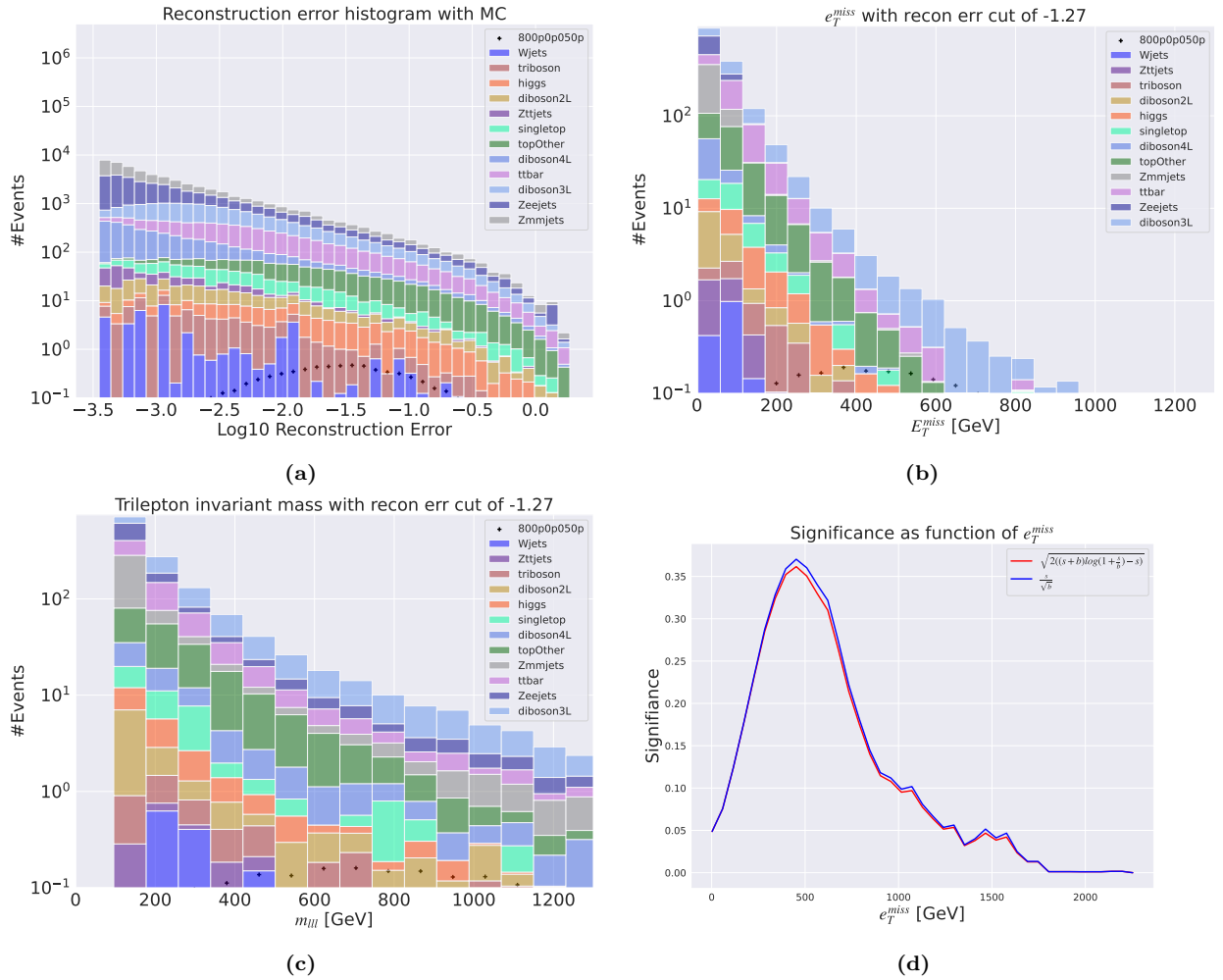
Figure 4.11: Reconstruction error, e_T^{miss} signal region, m_{III} signal region and significance as function of e_T^{miss} for the deep regular autoencoder using the SUSY 800p50. Figure 4.11a shows the reconstruction error distribution for the SM MC and the SUSY signal. Here the autoencoder produces a mirrored reconstruction error shape for background and signal. The peaks of the two distributions are separated with two orders of magnitude in reconstruction error. Figure 4.11b shows the e_T^{miss} distribution for the SM MC and the SUSY signal in the signal region, defined as the region having a \log_{10} reconstruction error above -1.27. Most of the background is removed, and the peaks of the SM MC and signal distributions are separated. Figure 4.11c shows the m_{III} distribution for the SM MC and the SUSY signal. The shape of the SM MC and the signal distributions are somewhat separated. Figure 4.11d shows the significance as function of e_T^{miss} . The maximum significance is found when applying a cut of about > 430 GeV in the e_T^{miss} , with a significance of around 0.37.
