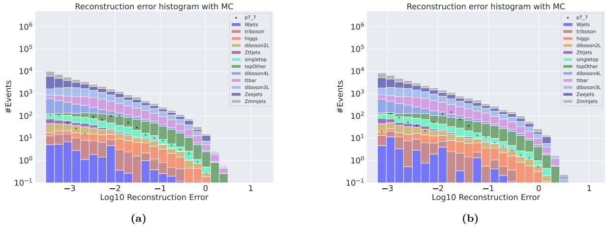
Figure 10: Reconstruction error on validation SM MC from the small (a) and large (b) regular autoencoder. The signal is a subsample of the validation set where the transverse momentum of the first electron and the first muon has been increased with a scale of 7. The change of transverse energy has also been changed according to the scaling of transverse momentum. A small peak is found around 10^{-2} .
