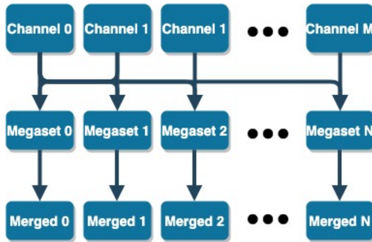
Figure 3.16: Megaset structure for the 2lep dataset. This figure generalises to M channels, and N megasets, where M and N does not have to be equal. The more you increase the number of megasets, the smaller each megaset will be in bytesize, but in order to keep the natural distribution in the SM MC distribution, it is not recommended to make too small sets. In this thesis 10 megasets were created where the simulated data contained 7 channels.
