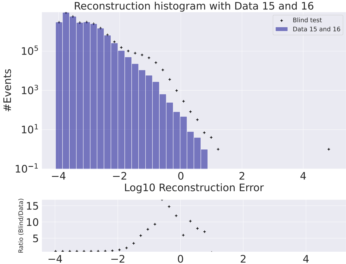
Figure 4.25: Reconstruction error for the blind test. The blue histogram is the ATLAS data 15 and data 16 sample and the black crosses are the ATLAS data mixed with BSM samples. Between a reconstruction error of 10^{-2} and 10^{0.5} there is a separation of the peaks of the two distributions. The biggest difference is a ratio difference of around 15.
