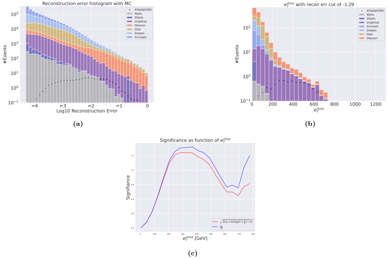
Figure 32: Reconstruction error (a), e_T^{miss} signal region (b) and significance as function of e_T^{miss} (c) for the deep regular autoencoder using SUSY 450p300. (a) shows the reconstruction error distribution for the SM MC and the SUSY signal. The autoencoder produces a slope like shape that is highly shifted to the lower end of the reconstruction error range for the background. The signal is more evenly spread out along the x-axis. The peaks of the two distributions are totally separated with two orders of magnitude in reconstruction error. (b) shows the e_T^{miss} T distribution for the SM MC and the SUSY signal in the signal region. The signal region is made using a cut around 10^{-1.29} . Most of the background is removed, and the peaks of the SM MC and signal distributions are somewhat separated. (c) shows the significance as function of e_T^{miss} . The peak is put around a cut of about 380 GeV in the e_T^{miss} , with a significance of around 1.3.
