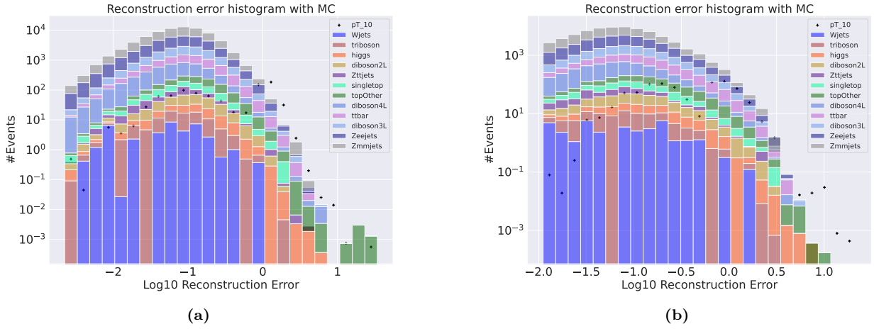
Figure 4.8: Reconstruction error on validation SM MC from the small (a) and large (b) variational autoencoder. The signal is a subsample of the validation set where the transverse momentum of the first electron and the first muon has been increased with a scale of 10. The difference in transverse energy between the objects has also been changed according to the scaling of transverse momentum. A peak is found around 10^{-1.6} .
