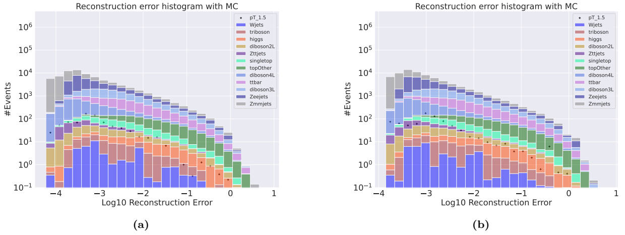
Figure 7: Reconstruction error on validation SM MC from the small (a) and large (b) regular autoencoder. The signal is a subsample of the validation set where the transverse momentum of the first electron and the first muon has been increased with a scale of 1.5. The change of transverse energy has also been changed according to the scaling of transverse momentum. A small peak is found around 10^{-3.3} .
