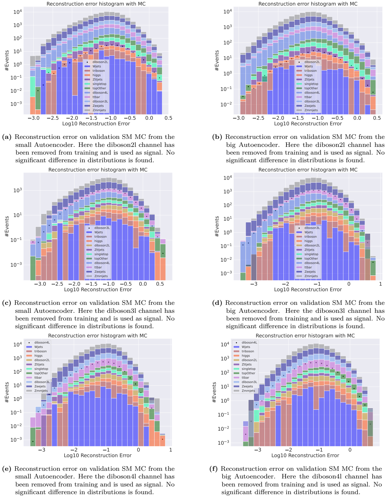
Figure 4: Reconstruction error on validation SM MC from the small and big Autoencoder. Here the diboson2l, diboson3l and diboson4l have been used for the small (left) and large (right) variational autoencoder
