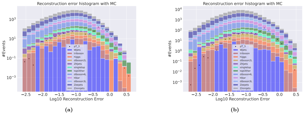
Figure 12: Reconstruction error on validation SM MC from the small (a) and large (b) variational autoencoder. The signal is a subsample of the validation set where the transverse momentum of the first electron and the first muon has been increased with a scale of 3. The change of transverse energy has also been changed according to the scaling of transverse momentum. A small peak is found around 10^{-0.5} .
