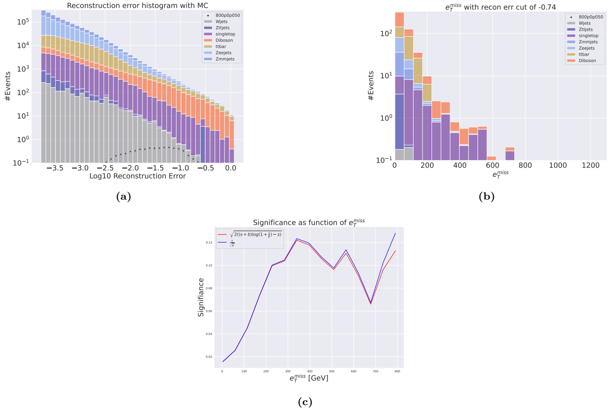
Figure 37: Reconstruction error (a), e_T^{\text{miss}} signal region (b) and significance as function of e_T^{\text{miss}} (c) for the deep regular autoencoder using SUSY 800p50. (a) shows the reconstruction error distribution for the SM MC and the SUSY signal. The autoencoder produces a slope like shape that is highly shifted to the lower end of the reconstruction error range for the background. The signal is more evenly spread out along the x-axis. The peaks of the two distributions are totally separated with two orders of magnitude in reconstruction error. (b) shows the e_T^{\text{miss}} T distribution for the SM MC and the SUSY signal in the signal region. The signal region is made using a cut around 10^{-0.74} . Most of the background is removed, and the peaks of the SM MC and signal distributions are somewhat separated. (c) shows the significance as function of e_T^{\text{miss}} . The peak is put around a cut of about 340 GeV in the e_T^{\text{miss}} , with a significance of around 0.125.
