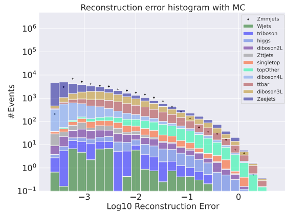
(c) Reconstruction error on validation SM MC from the small Autoencoder. Here the Zmmjets channel has been removed from training and is used as signal. No significant difference in distributions is found.
