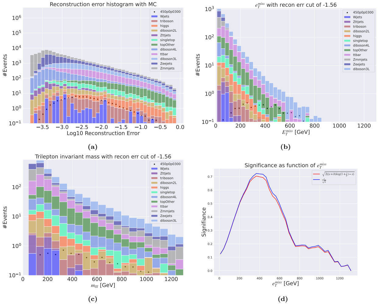
Figure 4.9: Reconstruction error, e_T^{miss} signal region, m_{III} signal region and significance as function of e_T^{miss} for the deep regular autoencoder using the SUSY 450p300. Figure 4.9a shows the reconstruction error distribution for the SM MC and the SUSY signal. Here the autoencoder produces the same reconstruction error shape for both background and signal. Figure 4.9b shows the e_T^{miss} distribution for the SM MC and the SUSY signal in the signal region, defined as the region having a \log_{10} reconstruction error above -1.56. Most of the background is removed, and the signal distribution is clearly shifted towards higher values of e_T^{miss} compared with SM MC. Figure 4.9c shows the m_{III} distribution for the SM MC and the SUSY signal. The shape of the SM MC and the signal distributions are too similar to distinguish. Figure 4.9d shows the significance as function of e_T^{miss} . The maximum significance is found when applying a cut of about > 380 GeV in the e_T^{miss} , with a significance of around 0.7.
