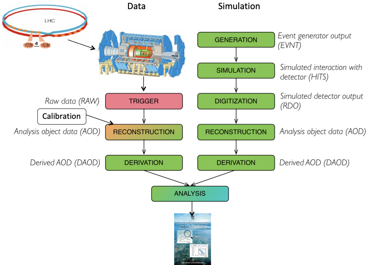
Figure 3.3: Figure describing the steps to take for data collection at ATLAS, fetched from Hybrid ATLAS Induction Day + Software Tutorial workshop , part Computing and Data preparation , initially drawn by Dr. James Catmore, later held by S.M Wang [26].
