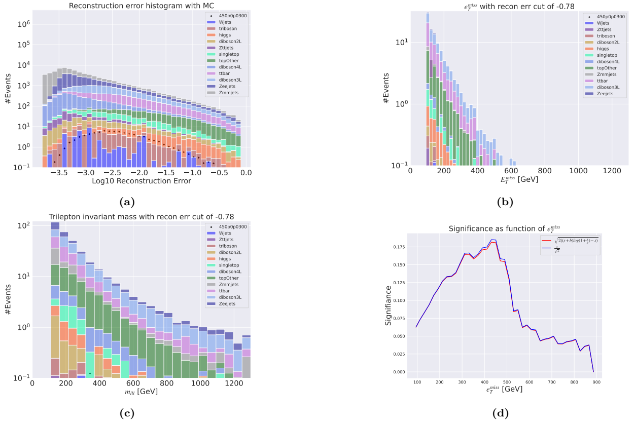
Figure 19: Reconstruction error, e_T^{\text{miss}} signal region, m_{lll} signal region and significance as function of e_T^{\text{miss}} for the deep regular autoencoder. Here the SUSY 450p300 model is used. Figure 19a shows the reconstruction error distribution for the SM MC and the SUSY signal. Here the autoencoder produce the same reconstruction error shape for both background and signal. Figure 19b shows the e_T^{\text{miss}} distribution for the SM MC and the SUSY signal in the signal region. The signal region is made using a cut around 10^{-0.78} . Most of the background is removed, with almost no signal in the signal region. Figure 19c shows the m_{lll} distribution for the SM MC and the SUSY signal. There is almost no signal in the signal region. Figure 19d shows the significance as function of e_T^{\text{miss}} . The peak is put around a cut of about 430 GeV in the e_T^{\text{miss}} , with a significance of around 0.185.
