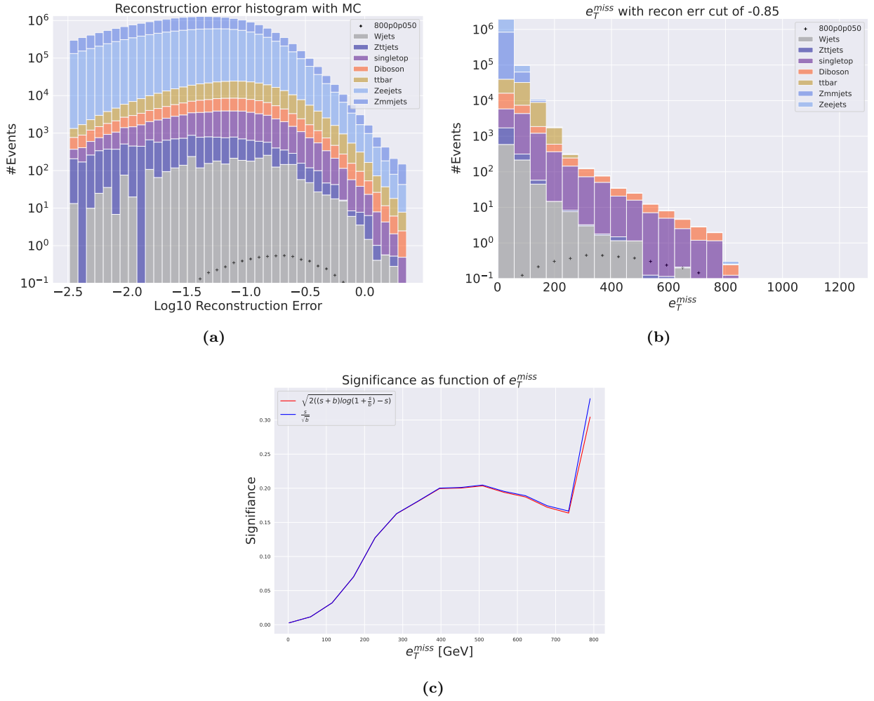
Figure 4.24: Reconstruction error (a), e_T^{miss} signal region (b) and significance as function of e_T^{miss} (c) for the shallow variational autoencoder using SUSY 800p50. (a) shows that the peak of the distribution is somewhat centered in the middle of the reconstruction error range forming a hill-like shape. The peaks of the background and signal distributions are not well separated, with almost identical reconstruction error pattern. (b) shows a signal region with large background distribution. The signal region is made using a cut around 10^{-0.72} . The peaks in the signal region are also somewhat separated, but the overall distributions are overlapping still. (c) shows the significance as function of e_T^{miss} .
