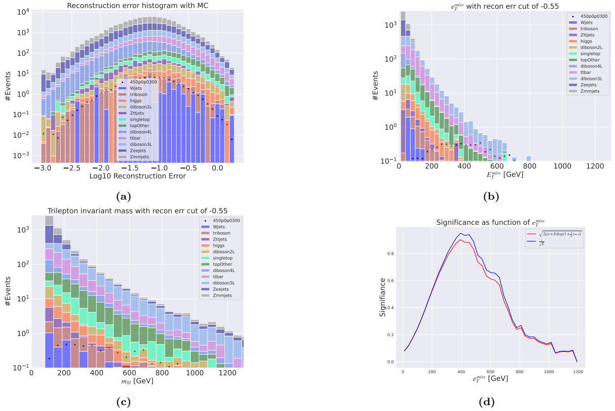
Figure 27: Reconstruction error, e_T^{\text{miss}} signal region, m_{lll} signal region and significance as function of e_T^{\text{miss}} for the deep variational autoencoder. Here the SUSY 450p300 model is used. Figure 27a shows the reconstruction error distribution for the SM MC and the SUSY signal. Here the autoencoder produce a bell-shape for background and signal with little distinction. The peaks of the two distributions are not separated in reconstruction error. Figure 27b shows the e_T^{\text{miss}} distribution for the SM MC and the SUSY signal in the signal region. The signal region is made using a cut around 10^{-0.55} . Some background is removed, and the peaks of the SM MC and signal distributions are separated. Figure 27c shows the m_{lll} distribution for the SM MC and the SUSY signal. The shape of both distributions are displaying almost the same shape. Figure 27d shows the significance as function of e_T^{\text{miss}} . The peak is put around a cut of about 400 GeV in the e_T^{\text{miss}} , with a significance of around 0.94.
