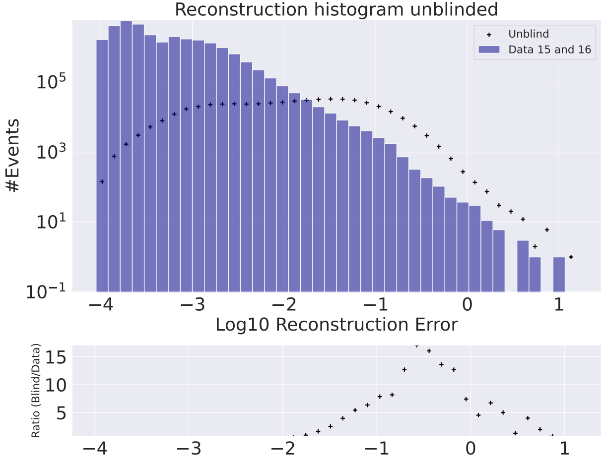
Figure 4.26: Reconstruction error for the unblind test. In the histogram the blue bins are the ATLAS data 15 and data 16 samples from the mix dataset and the black crosses are the BSM samples with the legend "Unblind". Between a reconstruction error of 10^{-2} and 10^{0.5} there is a separation of peaks of the two distributions. The biggest difference is a ratio difference of around 15.
