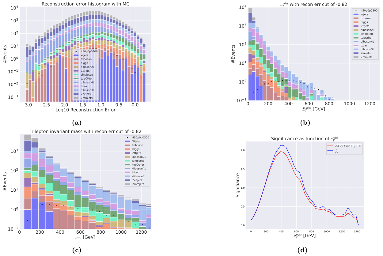
Figure 23: Reconstruction error, e_T^{miss} signal region, m_{lll} signal region and significance as function of e_T^{miss} for the deep variational autoencoder. Here the SUSY 450p300 model is used. Figure 23a shows the reconstruction error distribution for the SM MC and the SUSY signal. Here the autoencoder produce a bell-shape for background and signal with little distinction. The peaks of the two distributions are not separated in reconstruction error. Figure 23b shows the e_T^{miss} distribution for the SM MC and the SUSY signal in the signal region. The signal region is made using a cut around 10^{-0.82} . Some background is removed, and the peaks of the SM MC and signal distributions are separated. Figure 23c shows the m_{lll} distribution for the SM MC and the SUSY signal. The shape of both distributions are displaying almost the same shape. Figure 23d shows the significance as function of e_T^{miss} . The peak is put around a cut of about 400 GeV in the e_T^{miss} , with a significance of around 2.5.
