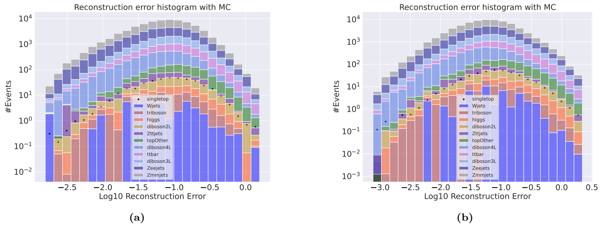
Figure 4.5: Reconstruction error on validation SM MC from the small (a) and large (b) variational autoencoder. The single top channel has been removed from training and is used as signal. No significant difference in distributions is found.
