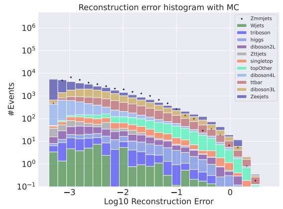
(d) Reconstruction error on validation SM MC from the big Autoencoder. Here the Zmmjets channel has been removed from training and is used as signal. No significant difference in distributions is found.
