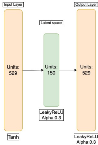
Figure 3.18: Small autoencoder architecture.
