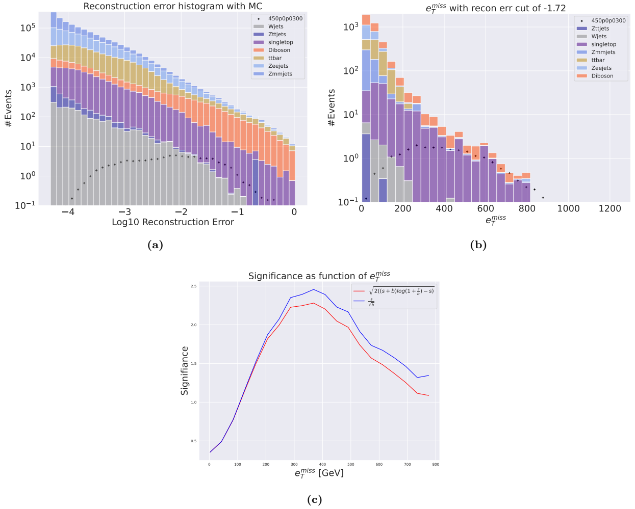
Figure 4.18: Reconstruction error (a), e_T^{\text{miss}} signal region (b) and significance as function of e_T^{\text{miss}} (c) for the shallow regular autoencoder using SUSY 450p300. (a) shows the reconstruction error distribution for the SM MC and the SUSY signal. The autoencoder produces a slope-like shape that is highly shifted to the lower end of the reconstruction error range for the background. The signal is more evenly spread out along the x-axis. The peaks of the two distributions are totally separated with two orders of magnitude in reconstruction error. (b) shows the e_T^{\text{miss}} T distribution for the SM MC and the SUSY signal in the signal region. The signal region is made using a cut around 10^{-1.72} . Most of the background is removed, and the peaks of the SM MC and signal distributions are somewhat separated. (c) shows the significance as function of e_T^{\text{miss}} . The peak is put around a cut of about 380 GeV in the e_T^{\text{miss}} , with a significance of around 2.4.
