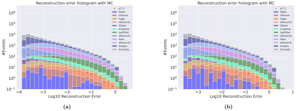
Figure 8: Reconstruction error on validation SM MC from the small (a) and large (b) regular autoencoder. The signal is a subsample of the validation set where the transverse momentum of the first electron and the first muon has been increased with a scale of 3. The change of transverse energy has also been changed according to the scaling of transverse momentum. A small peak is found around 10^{-2.8} .
