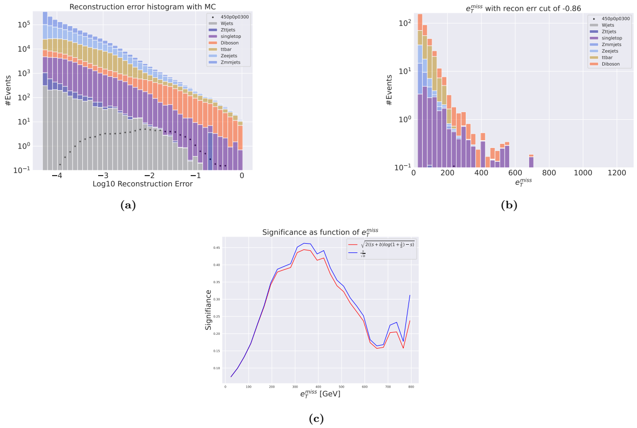
Figure 36: Reconstruction error (a), e_T^{miss} signal region (b) and significance as function of e_T^{miss} (c) for the deep regular autoencoder using SUSY 450p300. (a) shows the reconstruction error distribution for the SM MC and the SUSY signal. The autoencoder produces a slope like shape that is highly shifted to the lower end of the reconstruction error range for the background. The signal is more evenly spread out along the x-axis. The peaks of the two distributions are totally separated with two orders of magnitude in reconstruction error. (b) shows the e_T^{miss} T distribution for the SM MC and the SUSY signal in the signal region. The signal region is made using a cut around 10^{-0.86} . Most of the background is removed, and the peaks of the SM MC and signal distributions are somewhat separated. (c) shows the significance as function of e_T^{miss} . The peak is put around a cut of about 350 GeV in the e_T^{miss} , with a significance of around 0.47.
