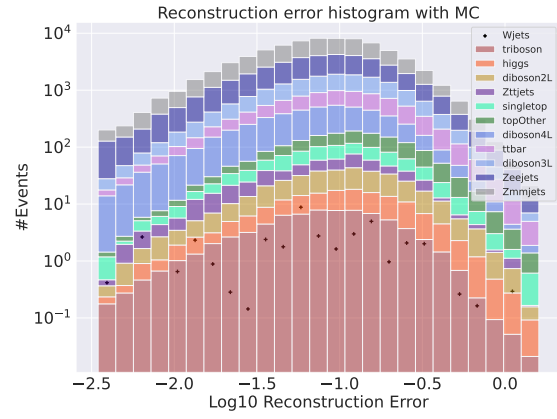
(a) Reconstruction error on validation SM MC from the small Autoencoder. Here the Wjets channel has been removed from training and is used as signal. No significant difference in distributions is found.
