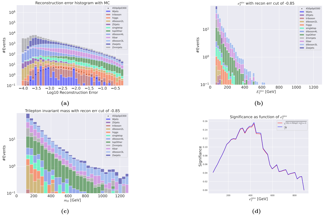
Figure 20: Reconstruction error, e_T^{miss} signal region, m_{lll} signal region and significance as function of e_T^{miss} for the shallow regular autoencoder. Here the SUSY 450p300 model is used. Figure 20a shows the reconstruction error distribution for the SM MC and the SUSY signal. Here the autoencoder produce the same reconstruction error shape for both background and signal. Figure 20b shows the e_T^{miss} distribution for the SM MC and the SUSY signal in the signal region. The signal region is made using a cut around 10^{-0.85} . Most of the background is removed, with almost no signal in the signal region. Figure 20c shows the m_{lll} distribution for the SM MC and the SUSY signal. There is almost no signal in the signal region. Figure 20d shows the significance as function of e_T^{miss} . The peak is put around a cut of about 430 GeV in the e_T^{miss} , with a significance of around 0.155.
