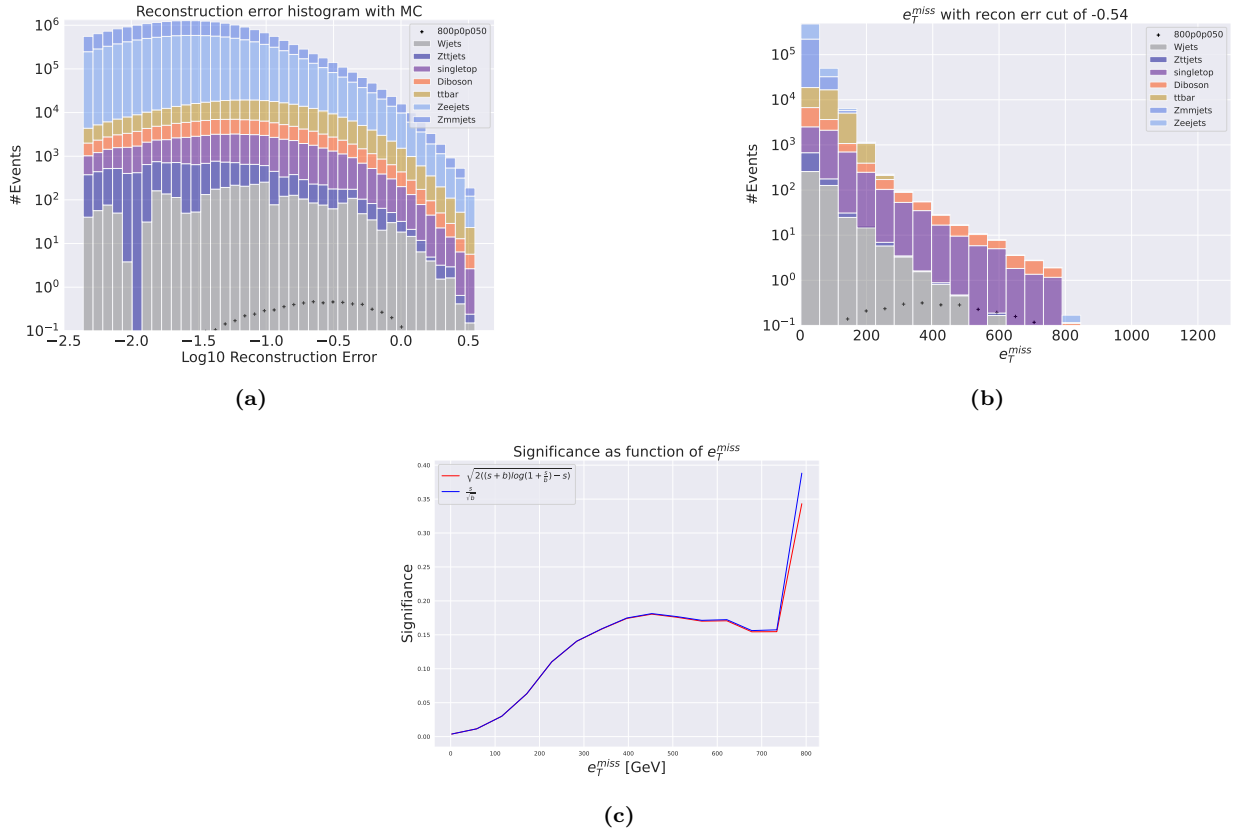
Figure 41: Reconstruction error (a), e_T^{\text{miss}} signal region (b) and significance as function of e_T^{\text{miss}} (c) for the deep regular autoencoder using SUSY 800p50. (a) shows that the peak of the distribution is somewhat centered in the middle of the reconstruction error range forming a bell-like shape. The peaks of the background and signal distributions are not well separated, with almost identical reconstruction error pattern. (b) shows a signal region with large background distribution. The signal region is made using a cut around 10^{-0.64} . The peaks in the signal region are also somewhat separated, but the overall distributions are overlapping still. (c) shows the significance as function of e_T^{\text{miss}} . The peak significance is around 1.35 at around 400 GeV.
