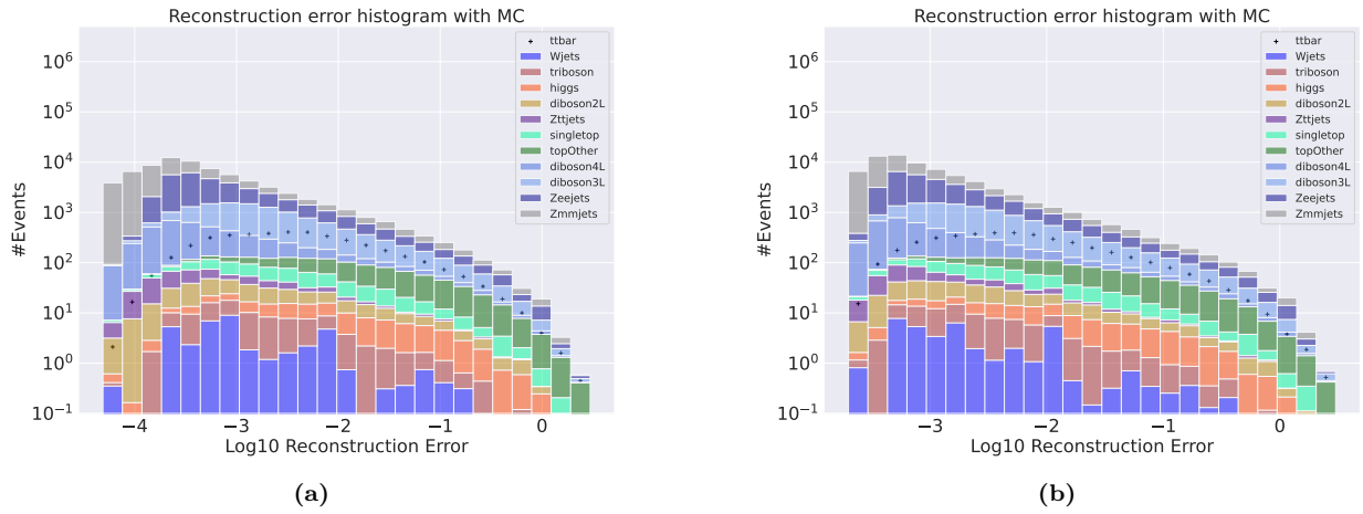
Figure 4.3: Reconstruction error on validation SM MC from the small (a) and large (b) autoencoder. The ttbar channel has been removed from training and is used as signal. No significant difference in distributions is found.
