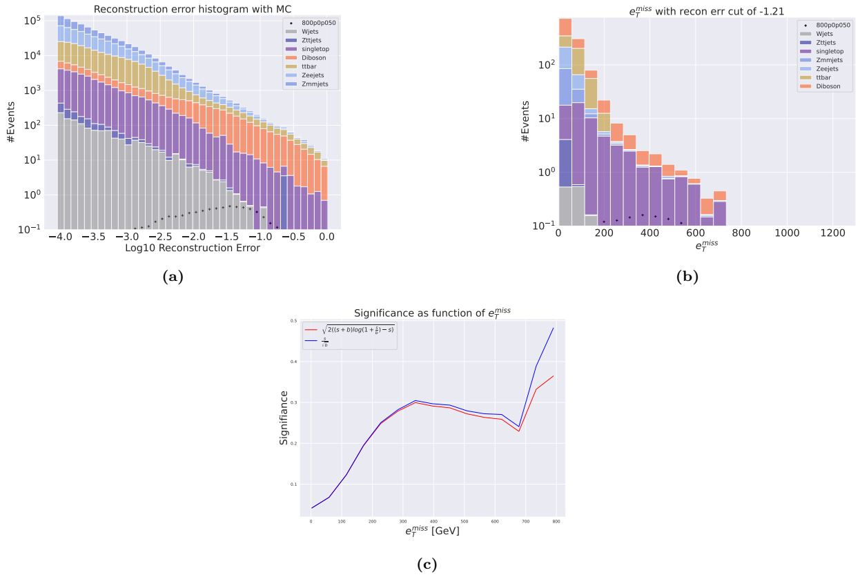
Figure 34: Reconstruction error (a), e_T^{miss} signal region (b) and significance as function of e_T^{miss} (c) for the deep regular autoencoder using SUSY 800p50. (a) shows the reconstruction error distribution for the SM MC and the SUSY signal. The autoencoder produces A slope like shape that is highly shifted to the lower end of the reconstruction error range for the background. The signal is more evenly spread out along the x-axis. The peaks of the two distributions are totally separated with two orders of magnitude in reconstruction error. (b) shows the e_T^{miss} T distribution for the SM MC and the SUSY signal in the signal region. The signal region is made using a cut around 10^{-1.21} . Most of the background is removed, and the peaks of the SM MC and signal distributions are somewhat separated. (c) shows the significance as function of e_T^{miss} . The peak is put around a cut of about 340 GeV in the e_T^{miss} , with a significance of around 0.31.
