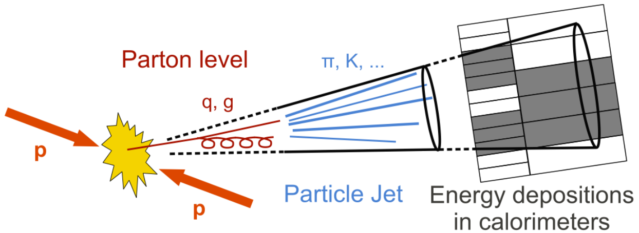
Figure 3.4: Figure describing how quarks and gluons are treated in the detector, and thus why we name them jets, fetched from the CMS webpage .
