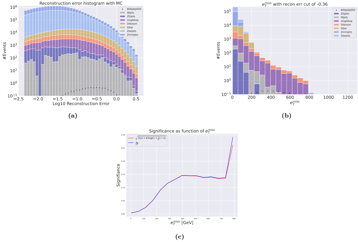
Figure 45: Reconstruction error (a), e_T^{\text{miss}} signal region (b) and significance as function of e_T^{\text{miss}} (c) for the deep regular autoencoder using SUSY 800p50. (a) shows that the peak of the distribution is somewhat centered in the middle of the reconstruction error range forming a bell-like shape. The peaks of the background and signal distributions are not well separated, with almost identical reconstruction error pattern. (b) shows a signal region with large background distribution. The signal region is made using a cut around 10^{-0.36} . The peaks in the signal region are also somewhat separated, but the overall distributions are overlapping still. (c) shows the significance as function of e_T^{\text{miss}} . The peak significance is around 0.148 at around 400 GeV.
