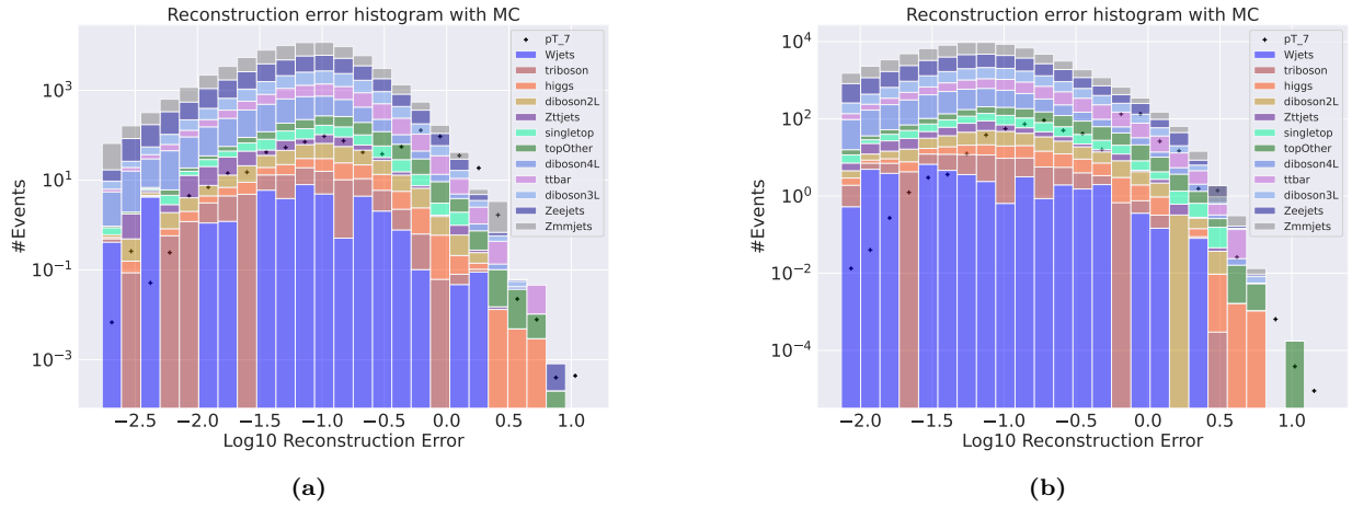
Figure 14: Reconstruction error on validation SM MC from the small (a) and large (b) variational autoencoder. The signal is a subsample of the validation set where the transverse momentum of the first electron and the first muon has been increased with a scale of 7. The change of transverse energy has also been changed according to the scaling of transverse momentum. A small peak is found around 10^{-0.3} .
