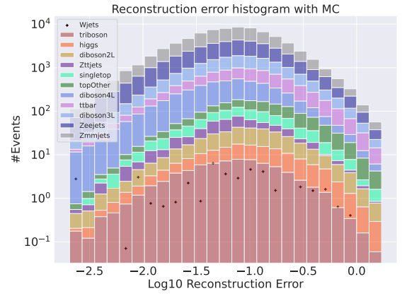
(b) Reconstruction error on validation SM MC from the big Autoencoder. Here the Wjets channel has been removed from training and is used as signal. No significant difference in distributions is found.
