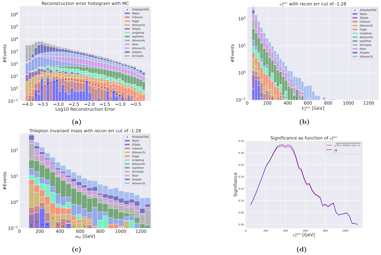
Figure 16: Reconstruction error, e_T^{miss} signal region, m_{lll} signal region and significance as function of e_T^{miss} for the shallow regular autoencoder. Here the SUSY 450p300 model is used. Figure 16a shows the reconstruction error distribution for the SM MC and the SUSY signal. Here the autoencoder produce the same reconstruction error shape for both background and signal. Figure 16b shows the e_T^{miss} distribution for the SM MC and the SUSY signal in the signal region. The signal region is made using a cut around 10^{-1.28} . Most of the background is removed, with almost no signal in the signal region. Figure 16c shows the m_{lll} distribution for the SM MC and the SUSY signal. There is almost no signal in the signal region. Figure 16d shows the significance as function of e_T^{miss} . The peak is put around a cut of about 380 GeV in the e_T^{miss} , with a significance of around 0.33.
