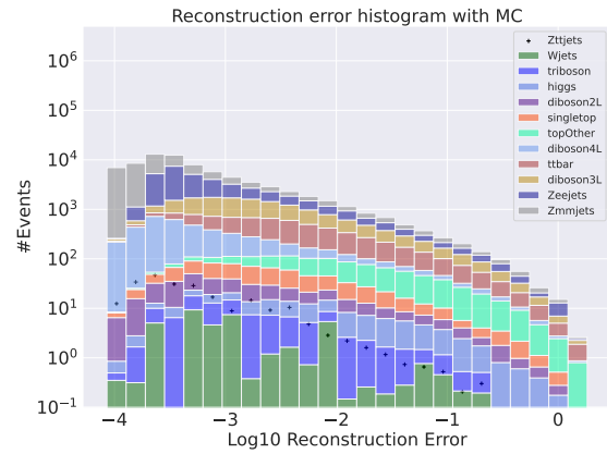
(e) Reconstruction error on validation SM MC from the small Autoencoder. Here the Zttjets channel has been removed from training and is used as signal. No significant difference in distributions is found.
