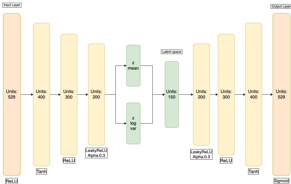
Figure 3.21: Large variational autoencoder architecture.
