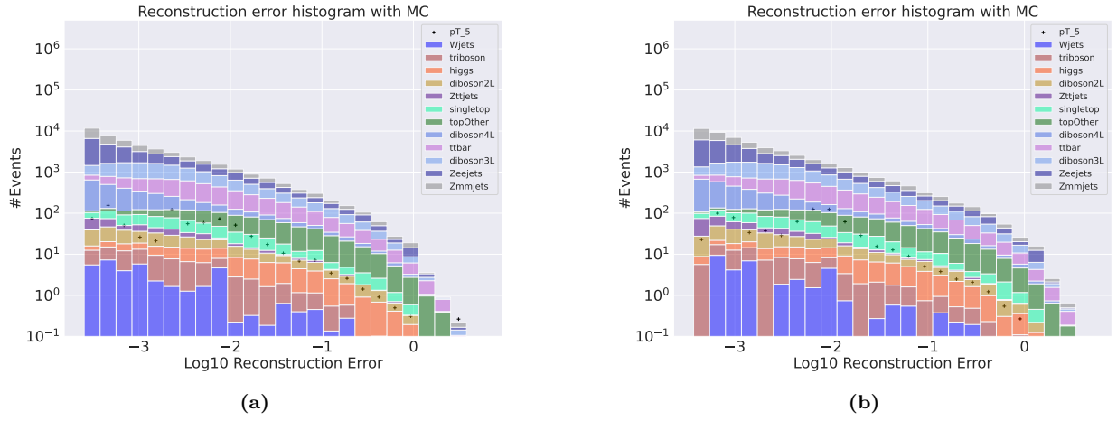
Figure 9: Reconstruction error on validation SM MC from the small (a) and large (b) regular autoencoder. The signal is a subsample of the validation set where the transverse momentum of the first electron and the first muon has been increased with a scale of 5. The change of transverse energy has also been changed according to the scaling of transverse momentum. A small peak is found around 10^{-2} .
