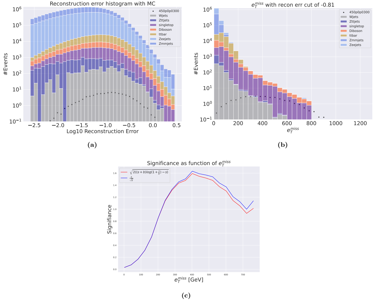
Figure 4.21: Reconstruction error (a), e_T^{miss} signal region (b) and significance as function of e_T^{miss} (c) for the deep variational autoencoder using SUSY 450p300. (a) shows that the peak of the distribution is somewhat centered in the middle of the reconstruction error range forming a hill-like shape. The peaks of the background and signal distributions are not well separated, with almost identical reconstruction error pattern. (b) shows a signal region with large background distribution. The signal region is made using a cut around 10^{-0.81} . The peaks in the signal region are also somewhat separated, but the overall distributions are overlapping still. (c) shows the significance as function of e_T^{miss} . The peak significance is around 1.61 at around 400 GeV.
