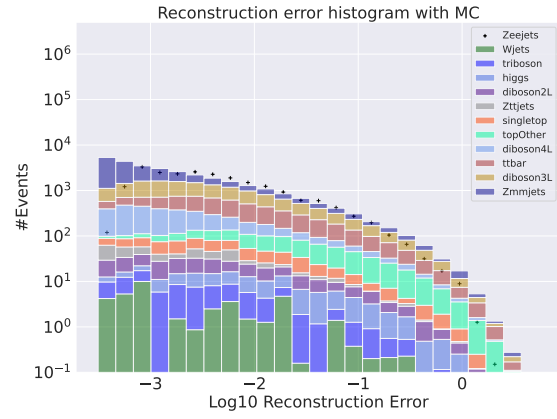
(a) Reconstruction error on validation SM MC from the small Autoencoder. Here the Zeejets channel has been removed from training and is used as signal. No significant difference in distributions is found.
