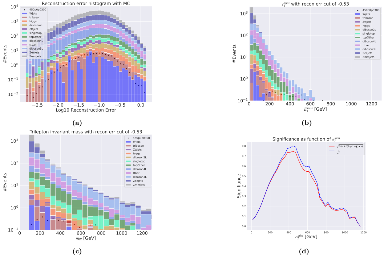
Figure 28: Reconstruction error, e_T^{miss} signal region, m_{lll} signal region and significance as function of e_T^{miss} for the shallow variational autoencoder. Here the SUSY 450p300 model is used. Figure 28a shows the reconstruction error distribution for the SM MC and the SUSY signal. Here the autoencoder produce a bell-shape for background and signal with little distinction. The peaks of the two distributions are not separated in reconstruction error. Figure 28b shows the e_T^{miss} distribution for the SM MC and the SUSY signal in the signal region. The signal region is made using a cut around 10^{-0.53} . Some background is removed, and the peaks of the SM MC and signal distributions are separated. Figure 28c shows the m_{lll} distribution for the SM MC and the SUSY signal. The shape of both distributions are displaying almost the same shape. Figure 28d shows the significance as function of e_T^{miss} . The peak is put around a cut of about 450 GeV in the e_T^{miss} , with a significance of around 0.81.
