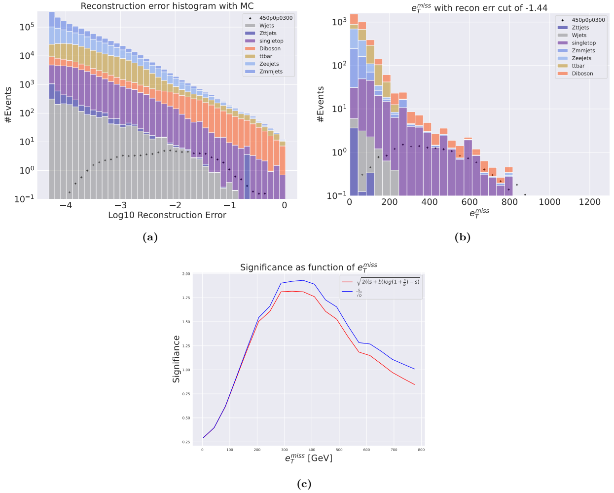
Figure 4.17: Reconstruction error (a), e_T^{miss} signal region (b) and significance as function of e_T^{miss} (c) for the deep regular autoencoder using SUSY 450p300. (a) shows the reconstruction error distribution for the SM MC and the SUSY signal. The autoencoder produces a slope-like shape that is highly shifted to the lower end of the reconstruction error range for the background. The signal is more evenly spread out along the x-axis. The peaks of the two distributions are totally separated with two orders of magnitude in reconstruction error. (b) shows the e_T^{miss} T distribution for the SM MC and the SUSY signal in the signal region. The signal region is made using a cut around 10^{-1.44} . Most of the background is removed, and the peaks of the SM MC and signal distributions are somewhat separated. (c) shows the significance as function of e_T^{miss} . The peak is put around a cut of about 380 GeV in the e_T^{miss} , with a significance of around 1.85.
