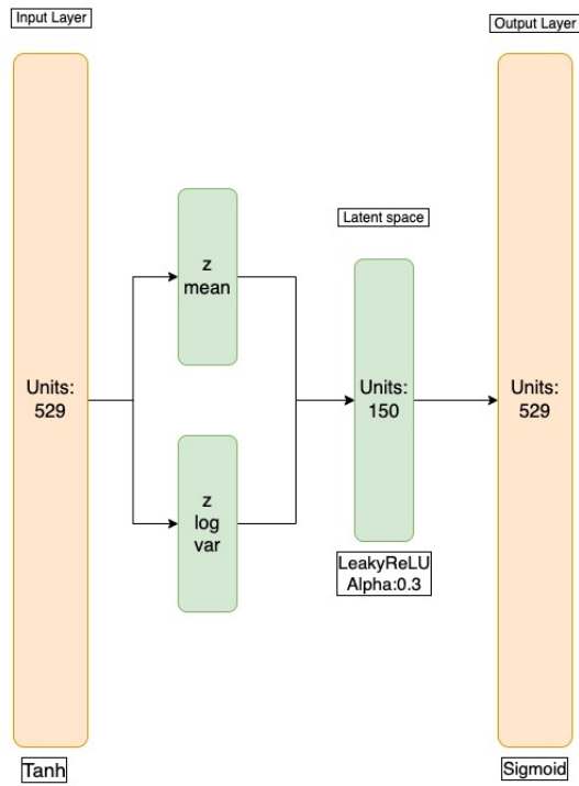
Figure 3.20: Small variational autoencoder architecture.
