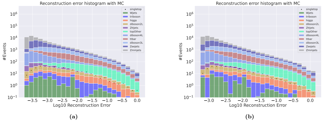
Figure 4.2: Reconstruction error on validation SM MC from the small (a) and large (b) autoencoders. The single top channel has been removed from training and is used as signal. No significant difference in distributions is found.
