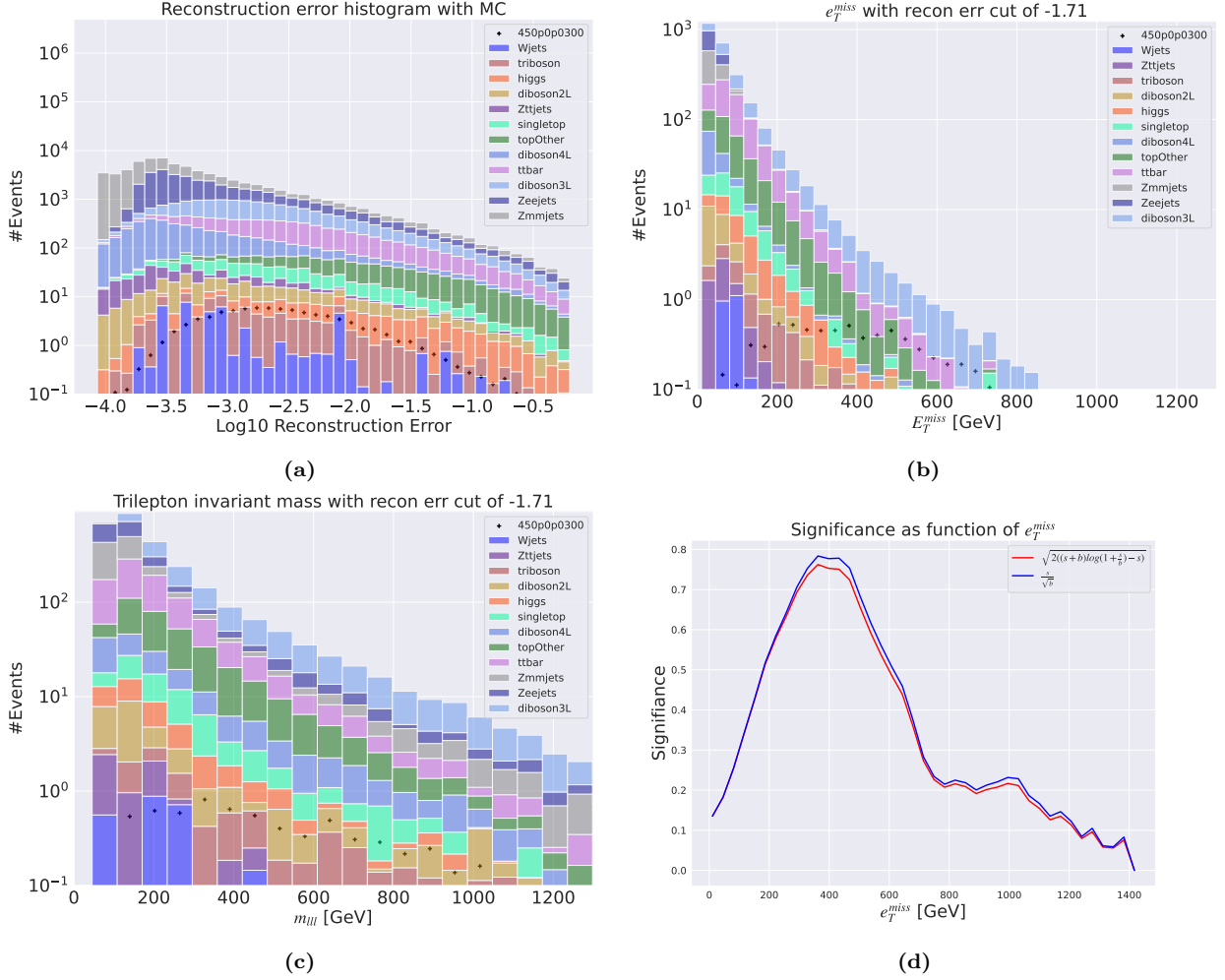
Figure 4.10: Reconstruction error, e_T^{miss} signal region, m_{lll} signal region and significance as function of e_T^{miss} for the shallow regular autoencoder using the SUSY 450p300 model. Figure 4.10a shows the reconstruction error distribution for the SM MC and the SUSY signal. Here the autoencoder produces the same reconstruction error shape for both background and signal, but with a small separation of the peaks of the distributions. Figure 4.10b shows the e_T^{miss} distribution for the SM MC and the SUSY signal in the signal region, defined as the region having a \log_{10} reconstruction error above -1.71. Most of the background is removed, and the peaks of the SM MC and signal distributions are somewhat separated. Figure 4.10c shows the m_{lll} distribution for the SM MC and the SUSY signal. The shape of the SM MC and the signal distributions are too similar to distinguish. Figure 4.10d shows the significance as function of e_T^{miss} . The maximum significance is found when applying a cut of about > 380 GeV in the e_T^{miss} , with a significance of around 0.78.
