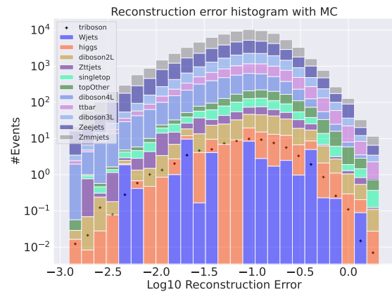
(e) Reconstruction error on validation SM MC from the small Autoencoder. Here the triboson channel has been removed from training and is used as signal. No significant difference in distributions is found.
