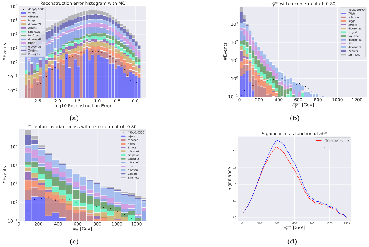
Figure 24: Reconstruction error, e_T^{miss} signal region, m_{lll} signal region and significance as function of e_T^{miss} for the shallow variational autoencoder. Here the SUSY 450p300 model is used. Figure 24a shows the reconstruction error distribution for the SM MC and the SUSY signal. Here the autoencoder produce a bell-shape for background and signal with little distinction. The peaks of the two distributions are not separated in reconstruction error. Figure 24b shows the e_T^{miss} distribution for the SM MC and the SUSY signal in the signal region. The signal region is made using a cut around 10^{-0.80} . Some background is removed, and the peaks of the SM MC and signal distributions are separated. Figure 24c shows the m_{lll} distribution for the SM MC and the SUSY signal. The shape of both distributions are displaying almost the same shape. Figure 24d shows the significance as function of e_T^{miss} . The peak is put around a cut of about 400 GeV in the e_T^{miss} , with a significance of around 2.6.
