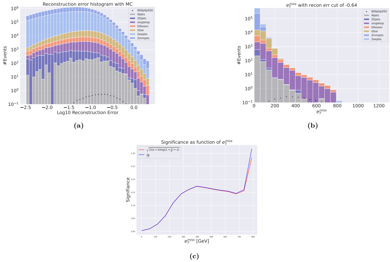
Figure 42: Reconstruction error (a), e_T^{miss} signal region (b) and significance as function of e_T^{miss} (c) for the deep regular autoencoder using SUSY 800p50. (a) shows that the peak of the distribution is somewhat centered in the middle of the reconstruction error range forming a bell-like shape. The peaks of the background and signal distributions are not well separated, with almost identical reconstruction error pattern. (b) shows a signal region with large background distribution. The signal region is made using a cut around 10^{-0.54} . The peaks in the signal region are also somewhat separated, but the overall distributions are overlapping still. (c) shows the significance as function of e_T^{miss} . The peak significance is around 0.17 at around 450 GeV.
