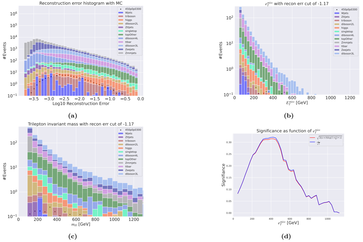
Figure 15: Reconstruction error, e_T^{\text{miss}} signal region, m_{lll} signal region and significance as function of e_T^{\text{miss}} for the deep regular autoencoder using the SUSY 450p300. Figure 15a shows the reconstruction error distribution for the SM MC and the SUSY signal. Here the autoencoder produce the same reconstruction error shape for both background and signal. Figure 15b shows the e_T^{\text{miss}} distribution for the SM MC and the SUSY signal in the signal region. The signal region is made using a cut around 10^{-1.17} . Most of the background is removed, with almost no signal in the signal region. Figure 15c shows the m_{lll} distribution for the SM MC and the SUSY signal. There is almost no signal in the signal region. Figure 15d shows the significance as function of e_T^{\text{miss}} . The peak is put around a cut of about 430 GeV in the e_T^{\text{miss}} , with a significance of around 0.35.
