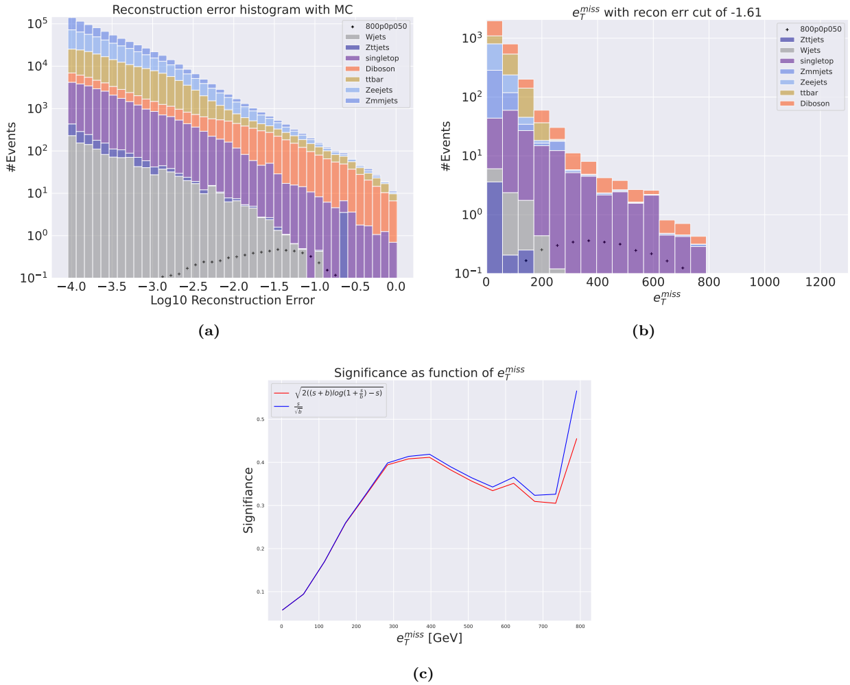
Figure 4.20: Reconstruction error (a), e_T^{miss} signal region (b) and significance as function of e_T^{miss} (c) for the shallow regular autoencoder using SUSY 800p50. (a) shows the reconstruction error distribution for the SM MC and the SUSY signal. The autoencoder produces a slope-like shape that is highly shifted to the lower end of the reconstruction error range for the background. The signal is more evenly spread out along the x-axis. The peaks of the two distributions are totally separated with two orders of magnitude in reconstruction error. (b) shows the e_T^{miss} T distribution for the SM MC and the SUSY signal in the signal region. The signal region is made using a cut around 10^{-1.61} . Most of the background is removed, and the peaks of the SM MC and signal distributions are somewhat separated. (c) shows the significance as function of e_T^{miss} . The peak is put around a cut of about 400 GeV in the e_T^{miss} , with a significance of around 0.42.
