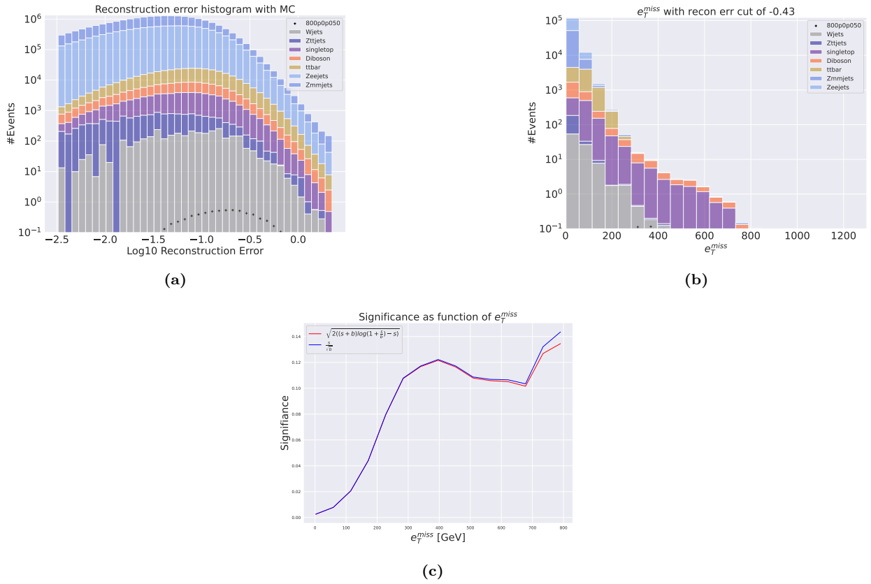
Figure 46: Reconstruction error (a), e_T^{miss} signal region (b) and significance as function of e_T^{miss} (c) for the deep regular autoencoder using SUSY 800p50. (a) shows that the peak of the distribution is somewhat centered in the middle of the reconstruction error range forming a bell-like shape. The peaks of the background and signal distributions are not well separated, with almost identical reconstruction error pattern. (b) shows a signal region with large background distribution. The signal region is made using a cut around 10^{-0.43} . The peaks in the signal region are also somewhat separated, but the overall distributions are overlapping still. (c) shows the significance as function of e_T^{miss} . The peak significance is around 0.123 at around 400 GeV.
