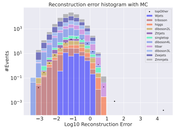
(d) Reconstruction error on validation SM MC from the big Autoencoder. Here the topOther channel has been removed from training and is used as signal. No significant difference in distributions is found.
