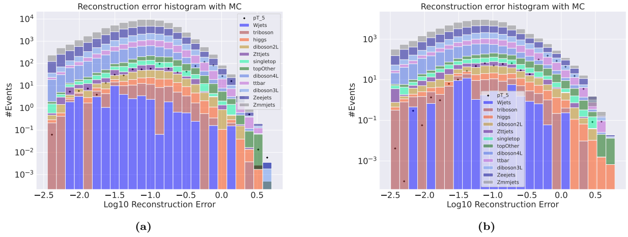
Figure 13: Reconstruction error on validation SM MC from the small (a) and large (b) variational autoencoder. The signal is a subsample of the validation set where the transverse momentum of the first electron and the first muon has been increased with a scale of 5. The change of transverse energy has also been changed according to the scaling of transverse momentum. A small peak is found around 10^{-0.3} .
