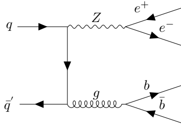
Figure 3.10: Proton-proton collision showing the Zeejets channel. Here one of the Z bosons decay leptonically and the gluon decays hadronically.
