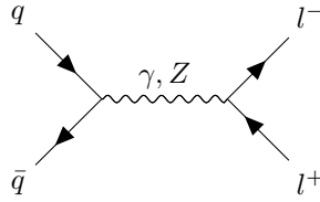
Figure 2.4: Proton-proton collision with lepton pair production via the Z boson or photon. Read from left to right.
