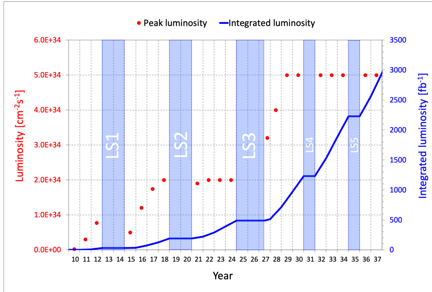
Figure 4.27: LHC nominal luminosity projections for the next 2 decades
