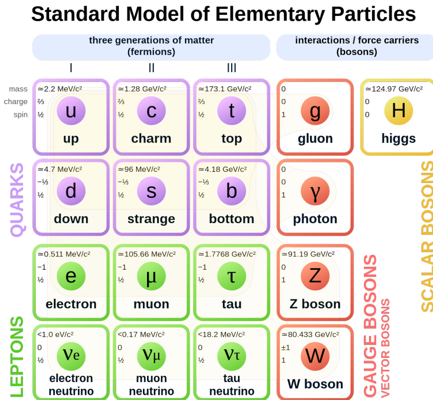
Figure 2.1: The SM of elementary particles. Source here . Accessed 07.10.22
