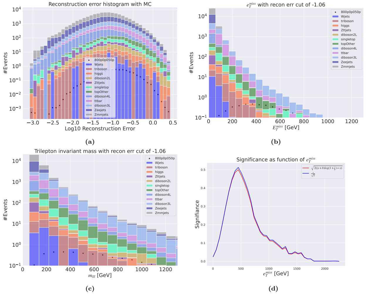
Figure 4.15: Reconstruction error, e_T^{miss} signal region, m_{III} signal region and significance as function of e_T^{miss} for the deep variational autoencoder using the SUSY 800p50. Figure 4.15a shows the reconstruction error distribution for the SM MC and the SUSY signal. Here the autoencoder produces a hill-like for background and signal with little distinction. The peaks of the two distributions are not separated in reconstruction error. Figure 4.15b shows the e_T^{miss} distribution for the SM MC and the SUSY signal in the signal region, defined as the region having a \log_{10} reconstruction error above -1.06. Some background is removed, and the peaks of the SM MC and signal distributions are separated. Figure 4.15c shows the m_{III} distribution for the SM MC and the SUSY signal. The shape of the SM MC and the signal distributions are displaying almost the same shape. Figure 4.15d shows the significance as function of e_T^{miss} . The maximum significance is found when applying a cut of about > 480 GeV in the e_T^{miss} , with a significance of around 0.6.
