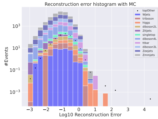
(c) Reconstruction error on validation SM MC from the small Autoencoder. Here the topOther channel has been removed from training and is used as signal. No significant difference in distributions is found.
