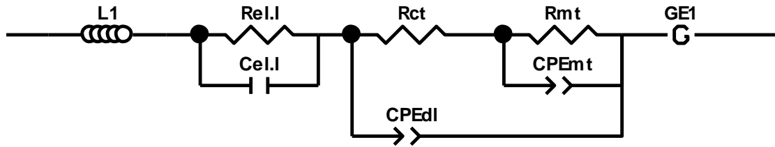
Figure 2. Equivalent circuit model, representing electrolyte resistance ( ReI.I ) and capacitance ( Cel.I ), charge transfer resistance ( Rct ) and double layer pseudo-capacitance ( CPEdI ), mass transfer resistance ( Rmt ) and pseudo-capacitance ( CPEmt ), and Gerischer impedance ( G ).
