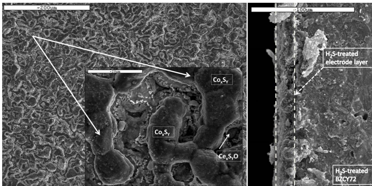
Figure 7. A) SEM pictures of the aged \text{Co}_3\text{O}_4/\text{CeO}_2 electrode at two different magnifications. B) Cross section image of the aged \text{Co}_3\text{O}_4-\text{CeO}_2/\text{BZCY72} interface.
