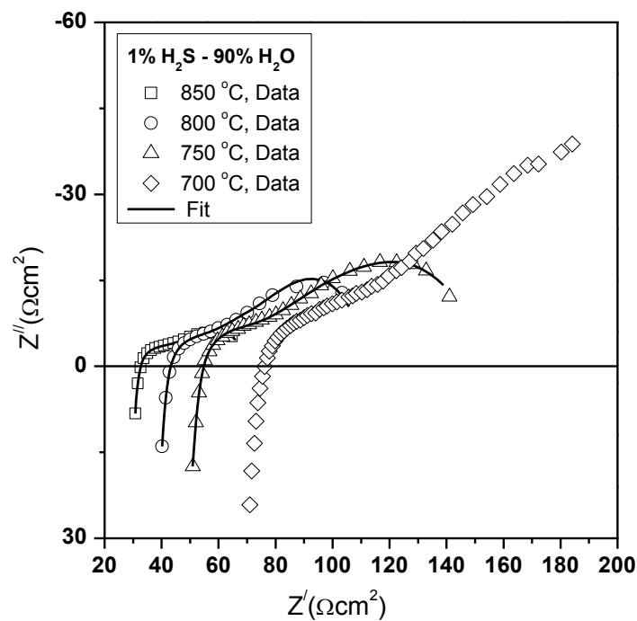
Figure 4. Impedance spectra and corresponding fitting curves as a function of cell temperature (700 – 850 °C). Reaction conditions: 1 v/v% H 2 S, 90 v/v% H 2 O diluted in Ar, F t =100 cm 3 /min.
