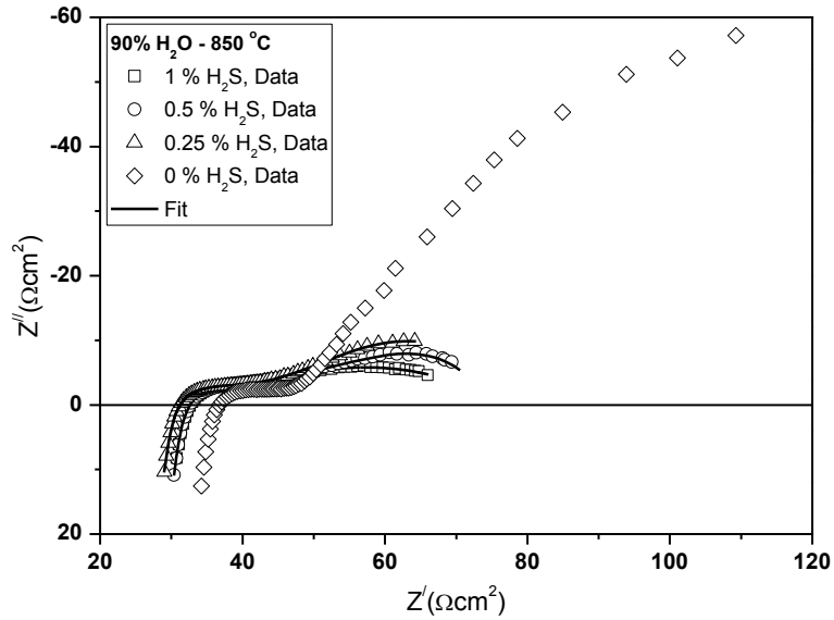
Figure 3. AC impedance spectra and corresponding fitting curves at different H 2 S concentrations. Reaction conditions: 0, 0.25, 0.5 and 1.0 v/v% H 2 S, 90 v/v% H 2 O diluted in Ar, F t = 100 cm 3 /min, T = 850 °C.
