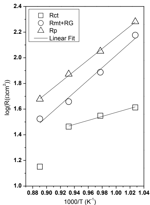
Figure 5. Arrhenius plots of electrode polarization, R_p , charge transfer, R_{ct} , and mass transfer, R_{mt} , resistances. Reaction conditions: 1 v/v% H_2S , 90 v/v% H_2O diluted in Ar, F_T = 100 \text{ cm}^3/\text{min}
