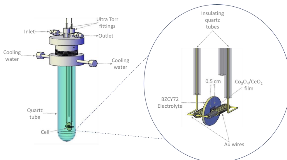
Figure 1. Schematic representation of the single chamber symmetrical proton conducting cell, \text{Co}_3\text{O}_4\text{-CeO}_2/\text{BZCY72}/\text{Co}_3\text{O}_4\text{-CeO}_2
