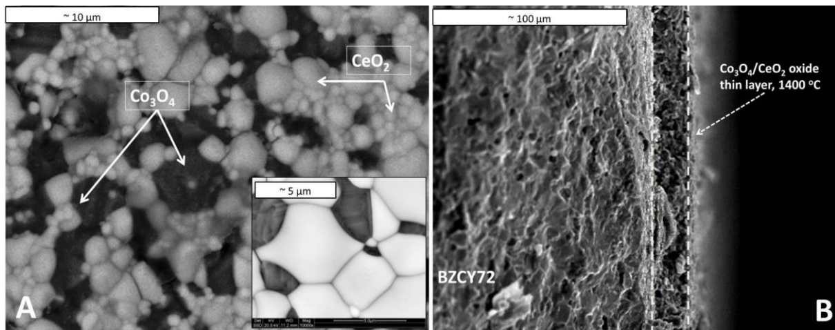
Figure 6. A) SEM pictures of the fresh calcined \text{Co}_3\text{O}_4/\text{CeO}_2 electrode surface at two different magnifications. B) Cross section image of the fresh \text{Co}_3\text{O}_4\text{-CeO}_2/\text{BZCY72} interface.
