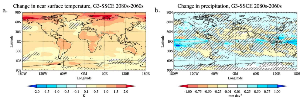
Figure 10. Termination effect. Simulated differences between G3-SSCE simulations averaged over the time period 2080–2089 minus the time period 2060–2069. Hatching denotes areas where the three models disagree on the sign of the change. (a) Near-surface temperature (K). (b) Precipitation ( \text{mm day}^{-1} ).
