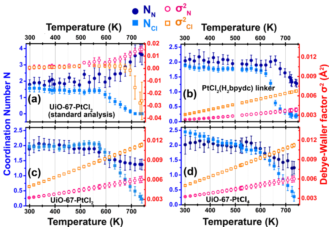
Figure 40. Part (a): standard analysis of the operando TPR-EXAFS series of spectra collected on UiO-67-bpy(PtCl 2 ). Each EXAFS spectrum has been analyzed as single datum, independently from the other spectra. In the (25-325) °C range, albeit relatively high error bars and some non-physical oscillations, reported values are meaningful. In the 325-475 °C range, reported values correspond to good mathematical fits of the experimental data, but has no meaningful physical interpretation. Parts (b)-(d): final refinement of the operando TPR-EXAFS experiments on PtCl 2 (H 2 bpydc) linker, UiO-67-bpy(PtCl 2 ) and UiO-67-bpy(PtCl 4 ), respectively. Data referring to the Pt–N and Pt–Cl bonds are reported as blue and cyan full-symbols and refer to the left ordinate axes. Corresponding Debye-Waller factors are reported as pink and orange open symbols and refer to the right ordinate axes.
