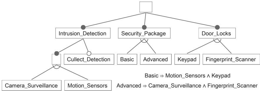
Figure 2.3: FODA Syntax Equivalent of Figure 2.2
