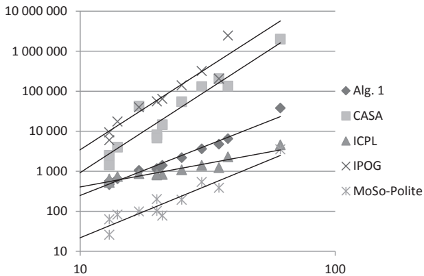
Figure C.3: Covering Array Sizes vs. Generation Time: 3-wise
