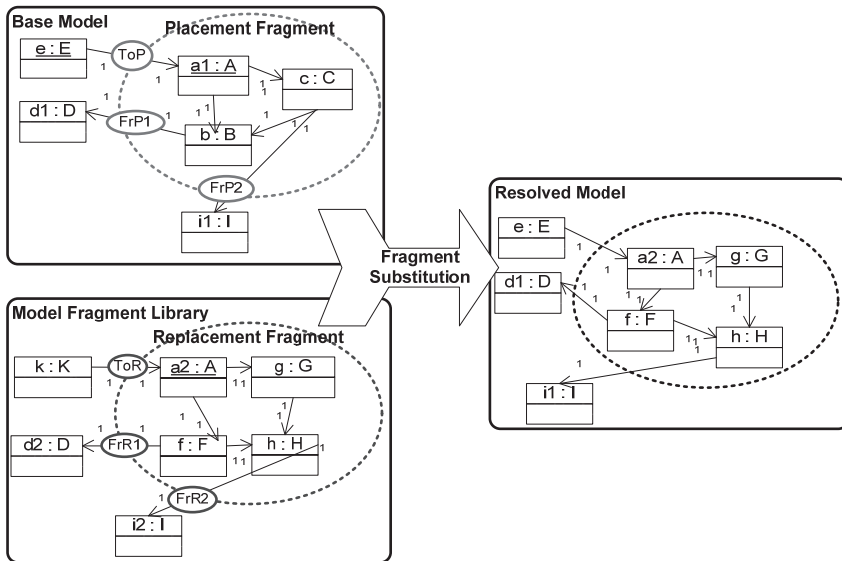
Figure 2.6: Fragment Substitution — From the CVL 1.2 User Guide [151]
