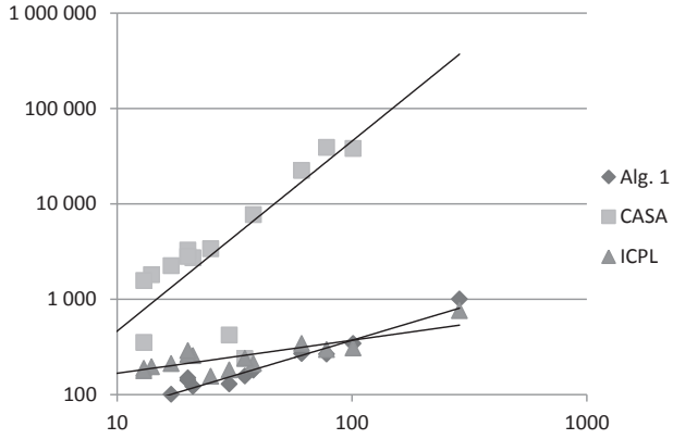
Figure C.1: Covering Array Sizes vs. Generation Time: 1-wise
