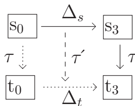
Figure 2.19: Incremental Testing as Described by [161]
