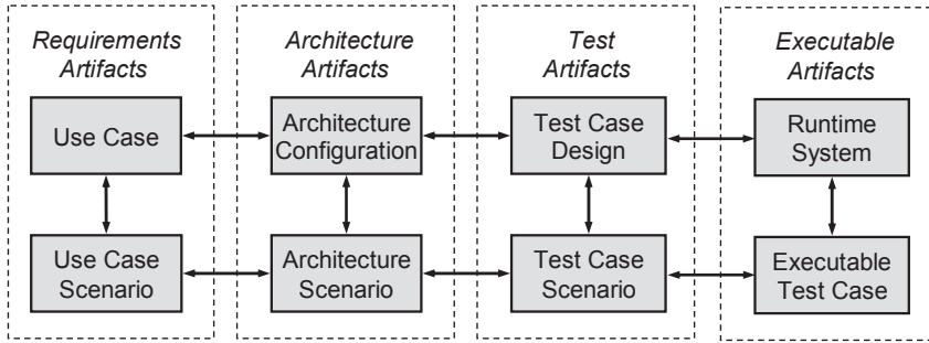
Figure 2.15: ScenTED Information Model – taken from [131]
