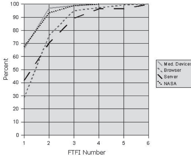
Figure 2.17: Faults Attributed to Interactions - taken from [94]
