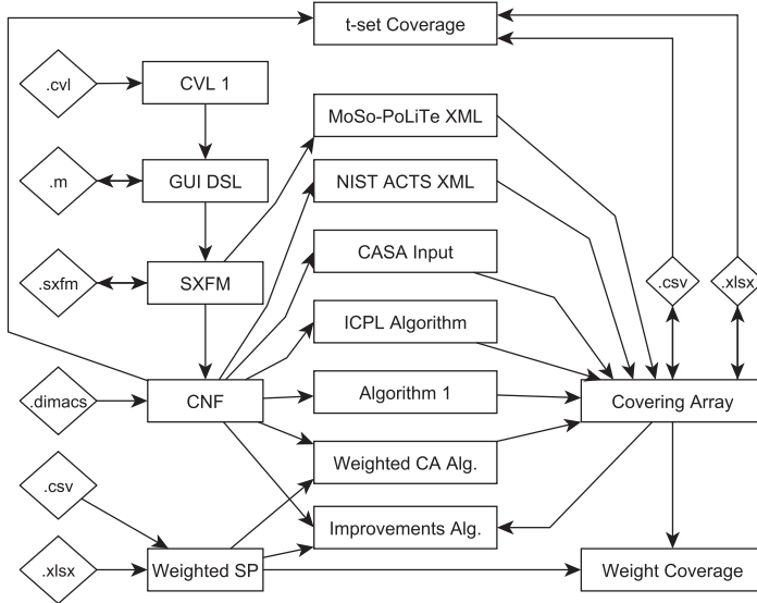
Figure D.1: Transformations in the Tool
