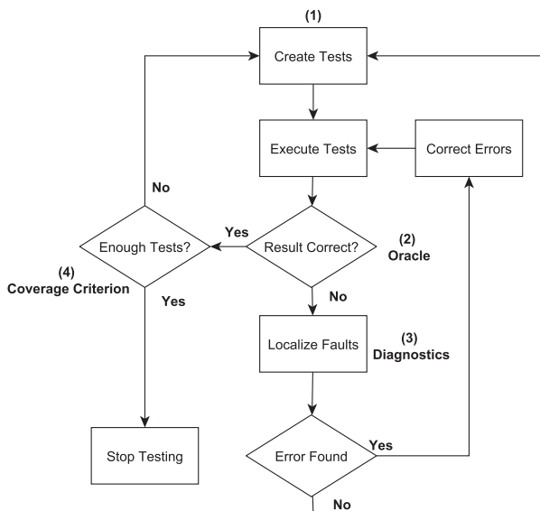
Figure 2.10: The Testing Process
