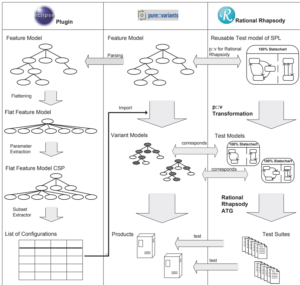
Figure 2.18: MoSo-PoLiTe Overview – taken from [115]
