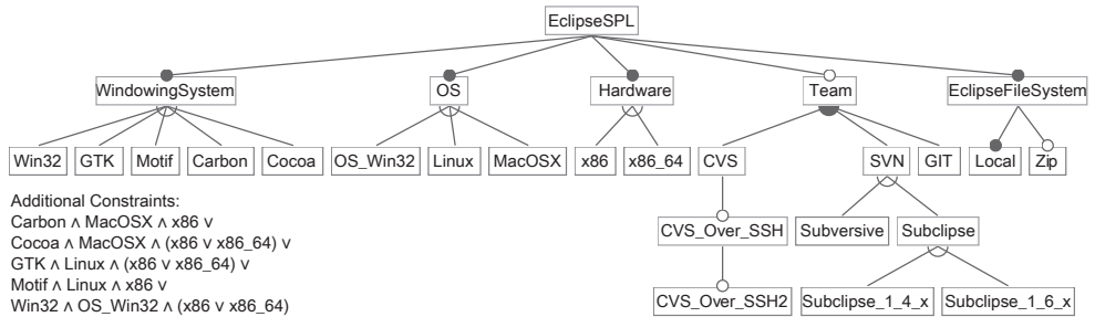
Figure 2.1: Feature model for a subset of Eclipse
