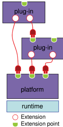
Figure 1.2: Overview of the Eclipse Plug-in System from [51]
