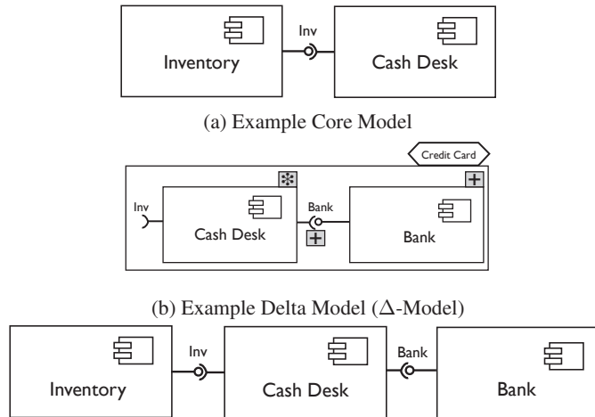
(c) Resulting Model From Applying the Delta Model in Figure 2.9b to the Core Model in Figure 2.9a
