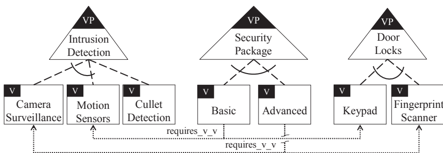
Figure 2.2: Orthogonal Variability Model — From [125]
