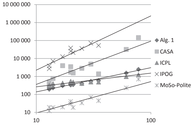
Figure C.2: Covering Array Sizes vs. Generation Time: 2-wise
