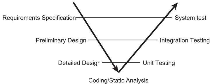
Figure 2.11: The V-Model
